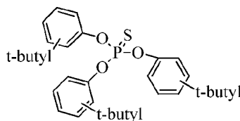
Butylated Triphenyl Phosphorothionate
