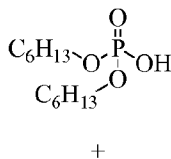
\text{C}_{13}\text{H}_{27}\sim\text{N}(\text{H})\sim\text{C}_{13}\text{H}_{27} Amine Phosphate + Ditridecyl Amine
