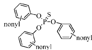
Nonyl Triphenyl Phosphorothionate
