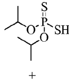
\text{C}_{13}\text{H}_{27}\sim\text{N}(\text{H})\sim\text{C}_{13}\text{H}_{27} Isopropyl Phosphorodithioate + Ditridecyl Amine
