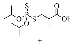
\text{C}_{13}\text{H}_{27}\sim\text{N}(\text{H})\sim\text{C}_{13}\text{H}_{27} Acidic Dialkyl Dithiophosphate + Ditridecyl Amine
