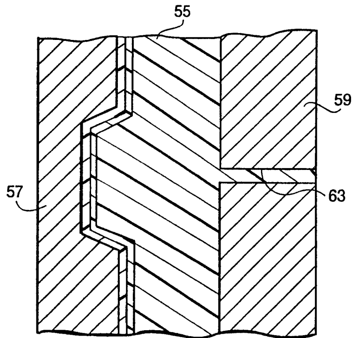
Fig. 9 (Prior Art)
