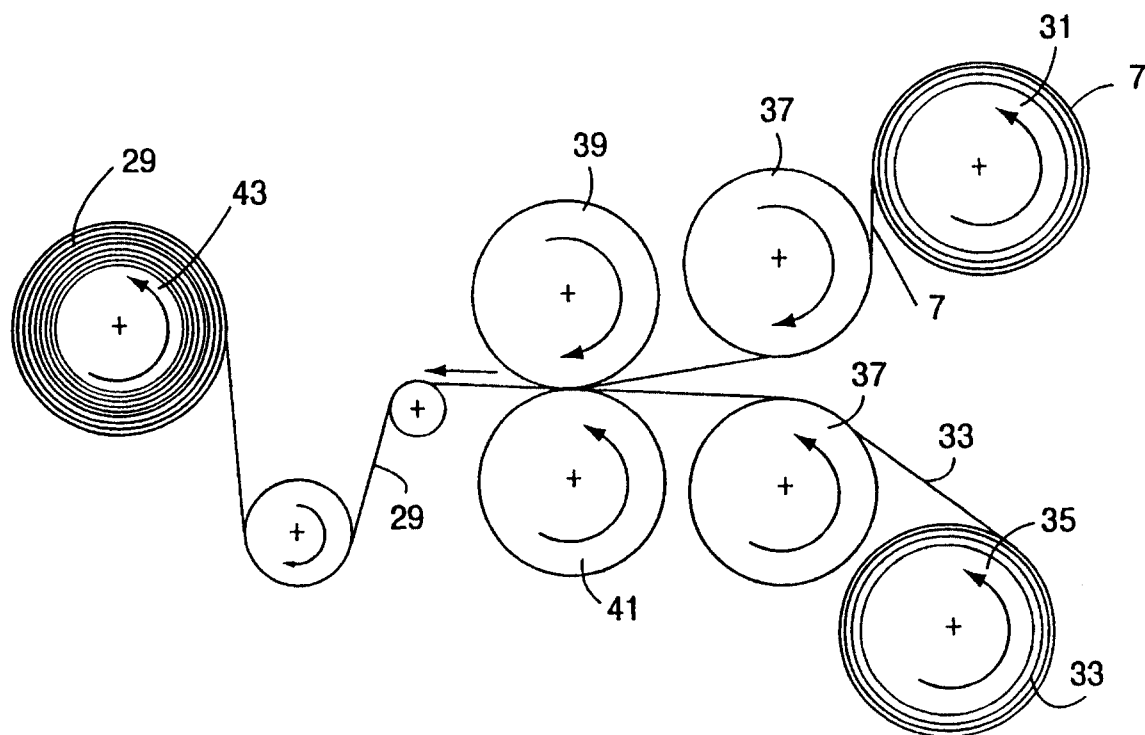
Fig. 4 (Prior Art)
