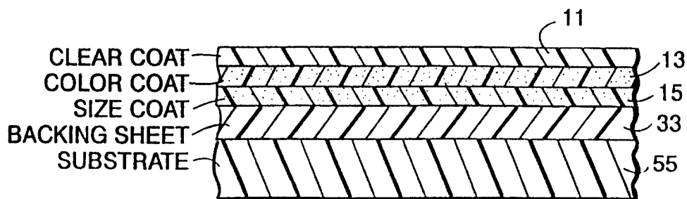
Fig. 10 (Prior Art)
