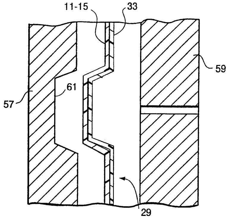
Fig. 8 (Prior Art)
