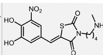
CPT-00213-02-01 ; [367.38]; 25 97% at 2 \mu M; 56% at 0.1 \mu M
