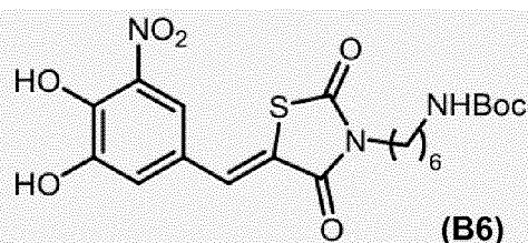
CPT-00347-01-01 ; [481.52]; 33 98% at 2 \mu M; 76% at 0.1 \mu M
