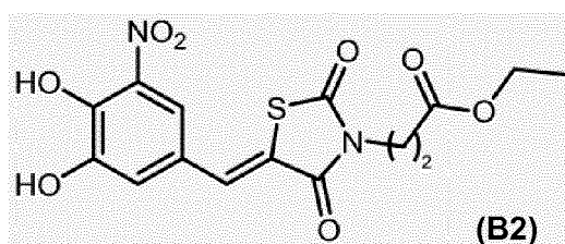
CPT-00346-01-01 ; [382.35]; 26 98% at 2 \mu M; 76% at 0.1 \mu M
