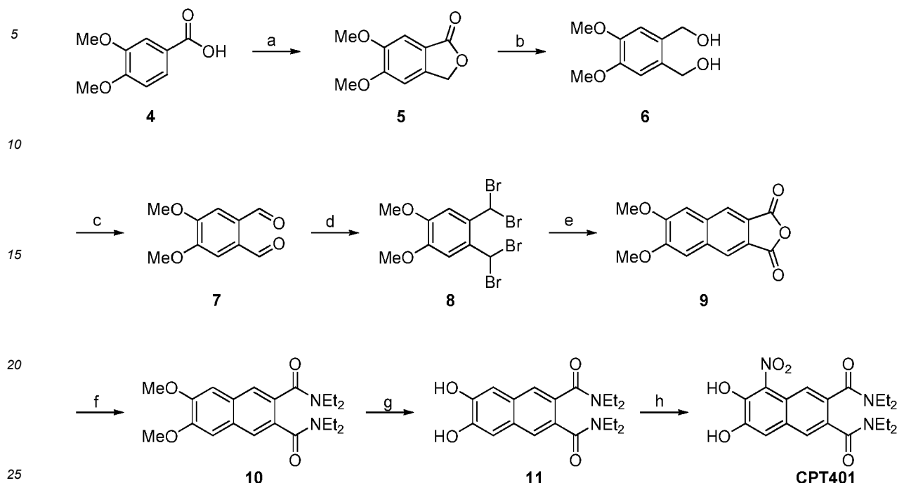
Scheme 2. Synthesis of novel COMT inhibitor CPT-401 (A1). Reagents and conditions: (a) formaldehyde, HCl (gas), 70 °C, 4 days, 93%; (b) LiAlH 4 , THF, 66 °C, 4 h, 77%; (c) oxalyl chloride, DMSO, TEA, DCM, -78 °C, 105 min → 23 °C, 60 min, 75%; (d) PBr 5 , benzene, 23 °C, 17 h, 41%; (e) maleic anhydride, NaI, DMF, 70 °C, 48 h, 69%; (f) diethyl amine, HATU, DIPEA, DMF, 23 °C, 48 h, 62%; (g) BBr 3 , DCM, 0 °C, 20 min → 23 °C, 60 min, 98%; (h) 2,3,5,6-tetrabromo-4-methyl-4-nitrocyclohexa-2,5-dienone, diethyl ether, 23 °C, 60 min, 55%.
