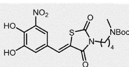
CPT-00345-01-01 ; [467.49]; 32 98% at 2 \mu M; 72% at 0.1 \mu M
