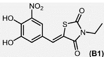
CPT-00212-01-01 ; [310.28]; 21 98% at 2 \mu M; 62% at 0.1 \mu M
