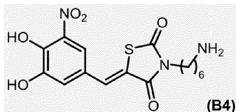
CPT-00349-01-01 ; [381.40]; 26 97% at 2 \mu M; 66% at 0.1 \mu M
