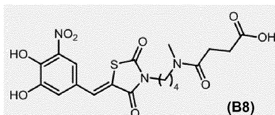
CPT-00348-01-01 ; [467.45]; 32 99% at 2 \mu M; 76% at 0.1 \mu M
