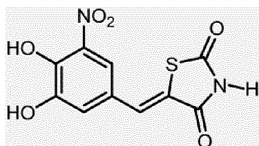
CPT-00342-01-01 ; [282.23]; 19 95% at 2 \mu M; 47% at 0.1 \mu M
