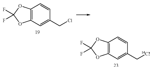
Scheme 4. Introduction of a radioactive isotope into Compound 1.
