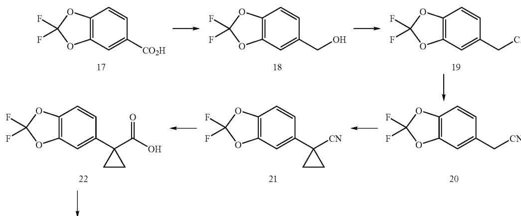
Scheme 1. Synthesis of the acid chloride moiety.
