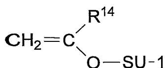
Formula (7)
