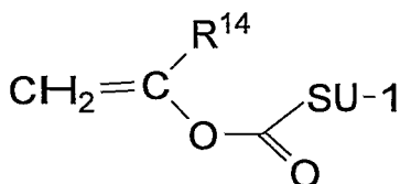
Formula (8)
