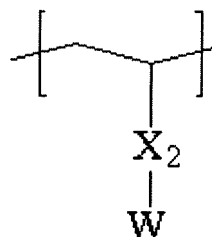
[Structural Formula 8]
