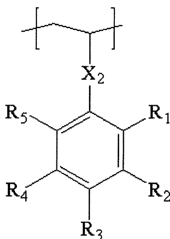
[Structural Formula 5]
