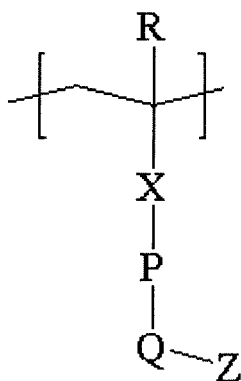
[Structural Formula 3]
