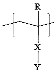
[Structural Formula 5]
