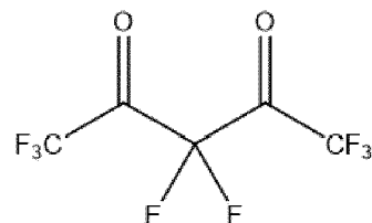
product
