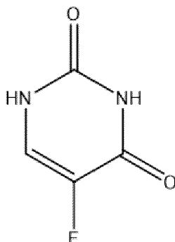
5-fluoro uracil product
