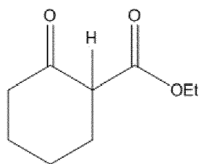
starting compound
