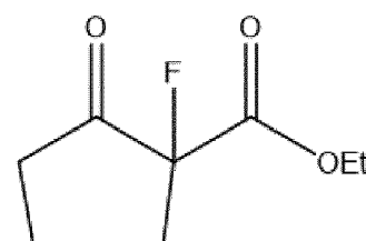
starting compound and product
