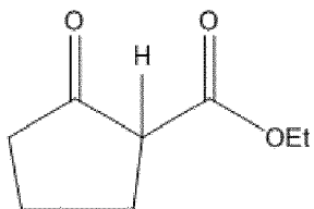
starting compound
