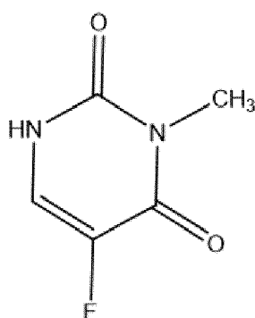
1-methyl-5-fluorouracil
