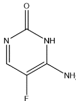
5-fluoro cytosine product
