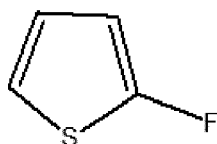
2-fluoro thiophene
