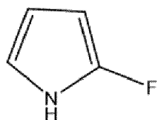
2-fluoro pyrrole
