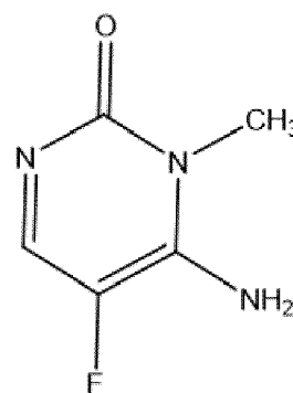
methylcytosine
