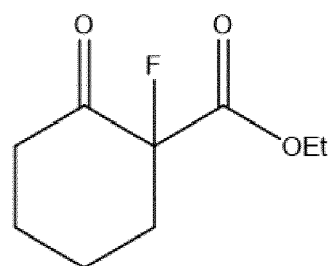
starting compound and product
