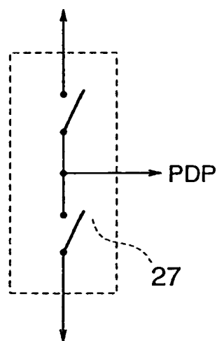
FIG. 6C (PRIOR ART)
