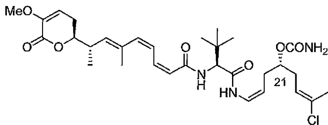
(21S)-Compound 1
