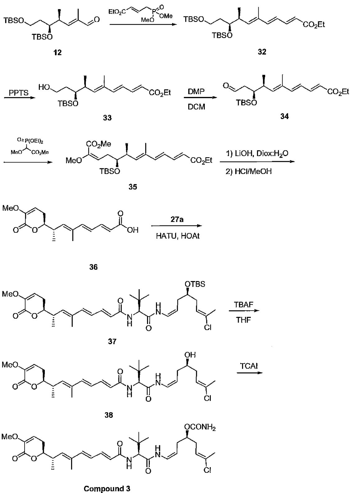
Scheme 6
