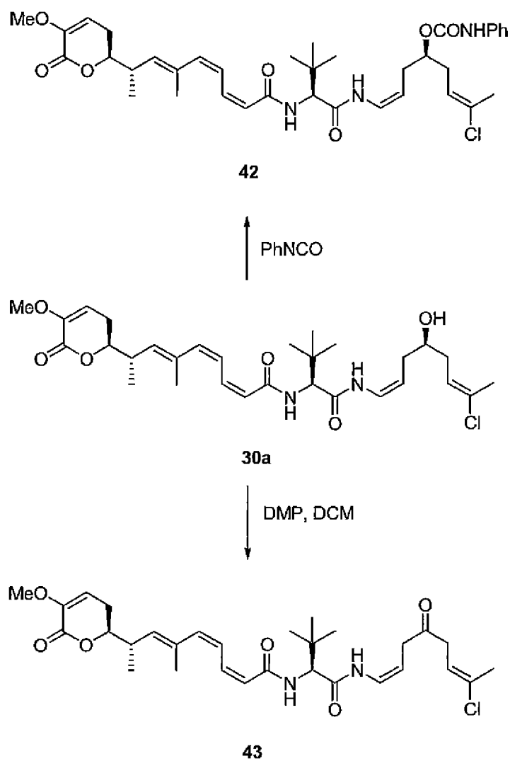
Scheme 8
