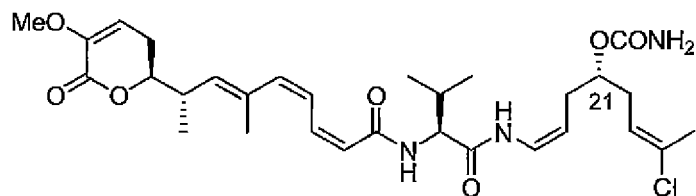
(21S)-Compound 5
