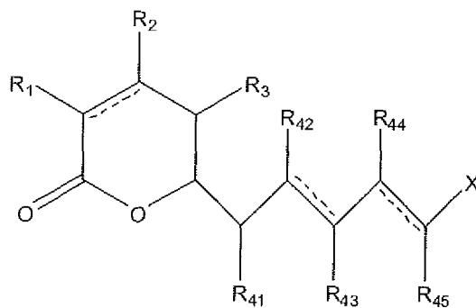
Fragment A
