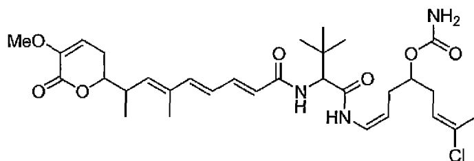
Compound 3
