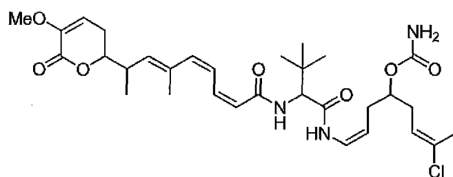
Compound 1
