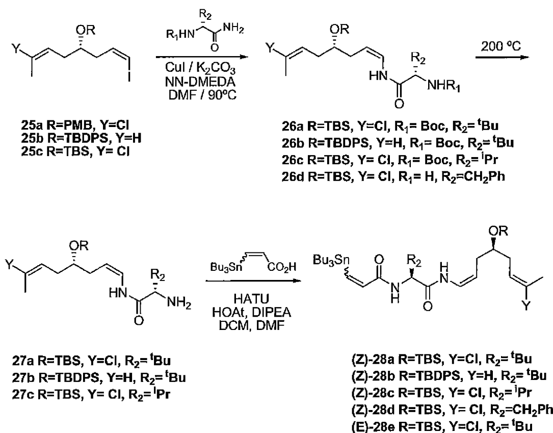
Scheme 4
