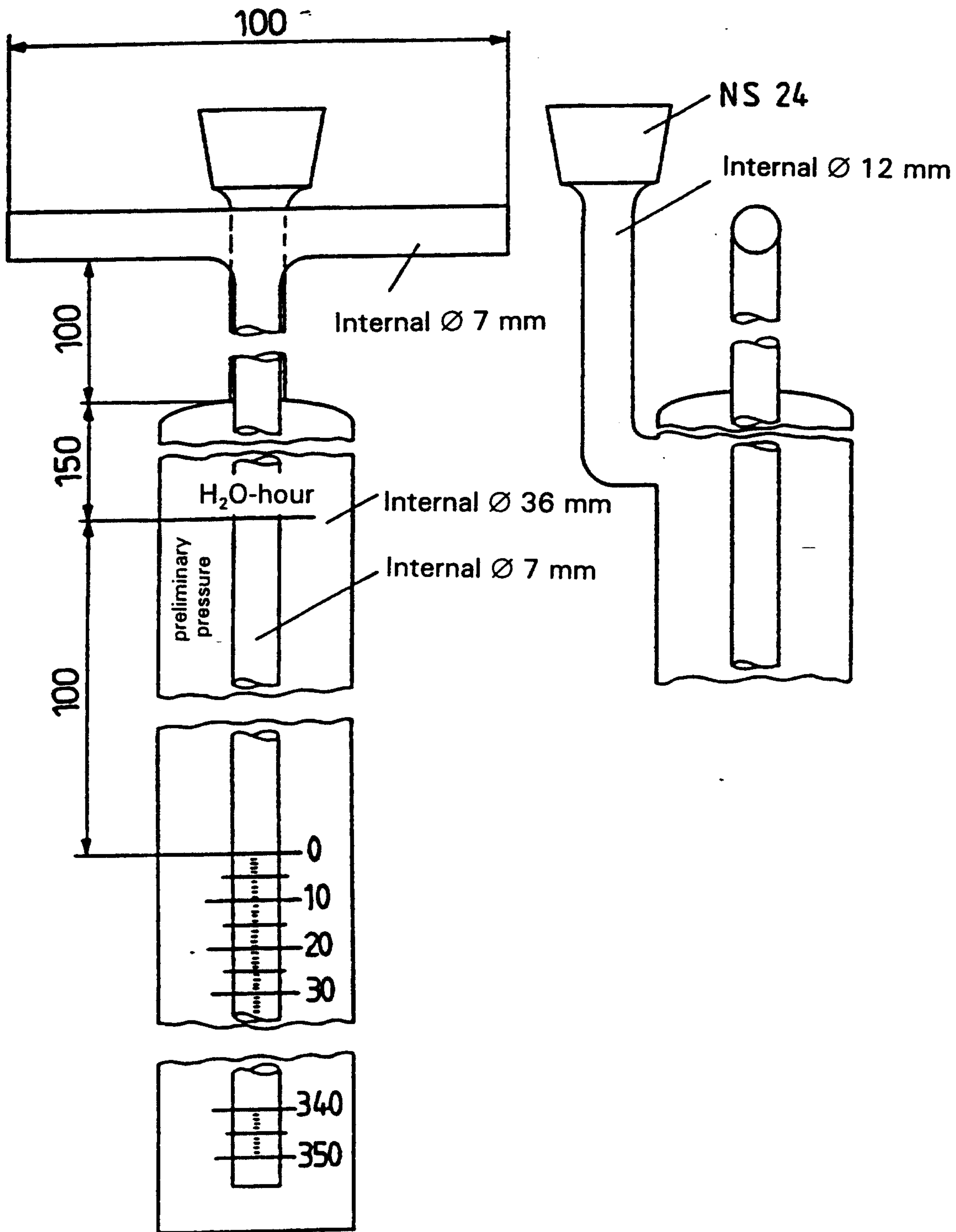
Glass vessel for flow resistance measurement apparatus
