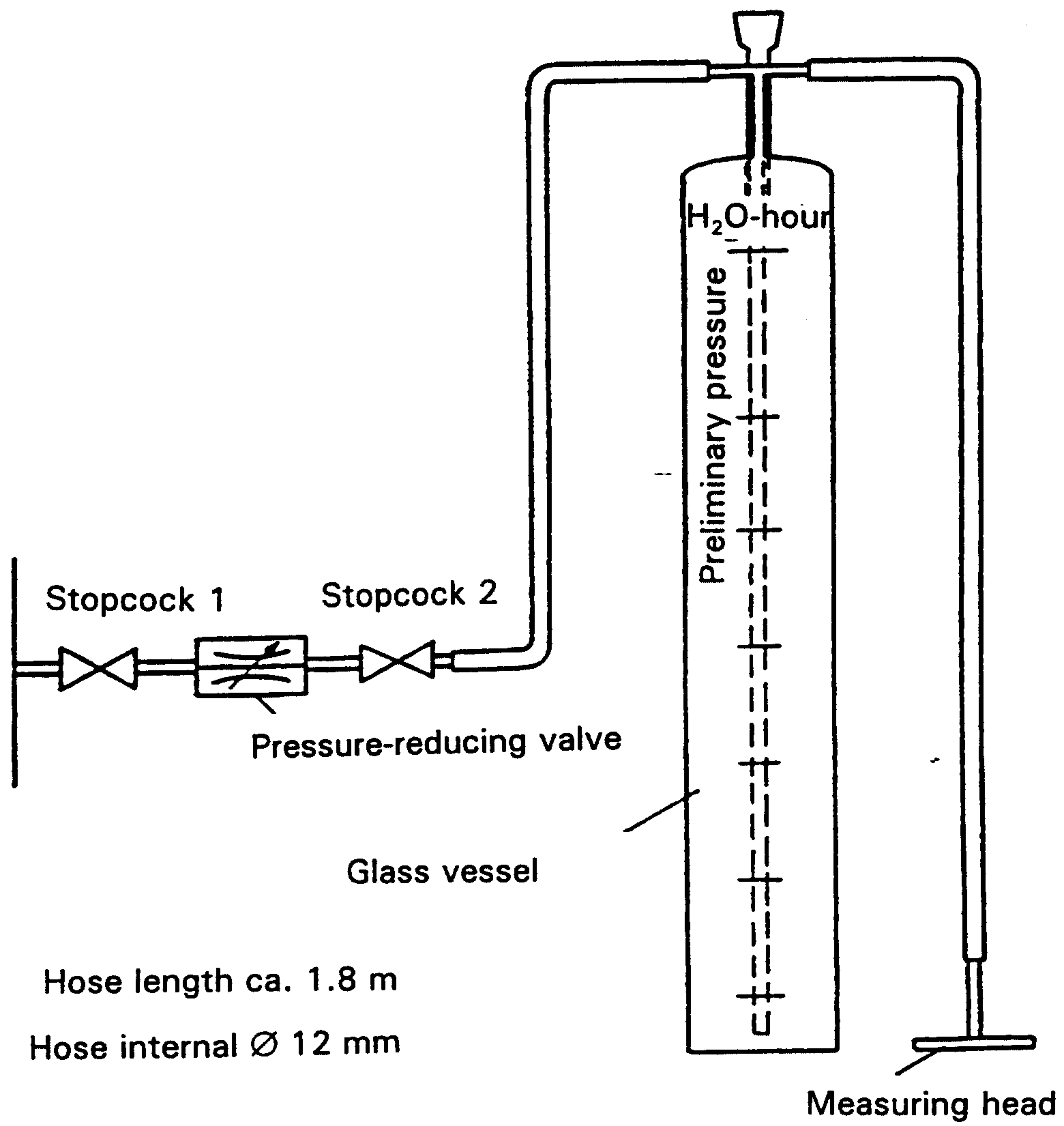
Flow resistance measurement apparatus
