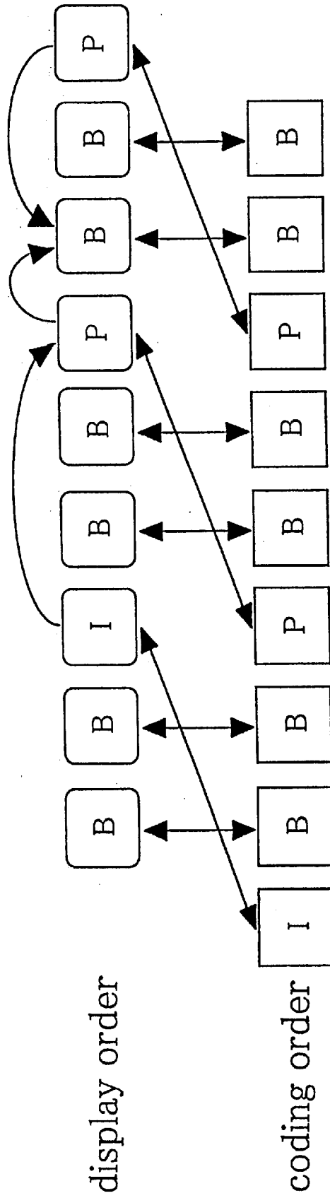
Fig.36 Prior Art
