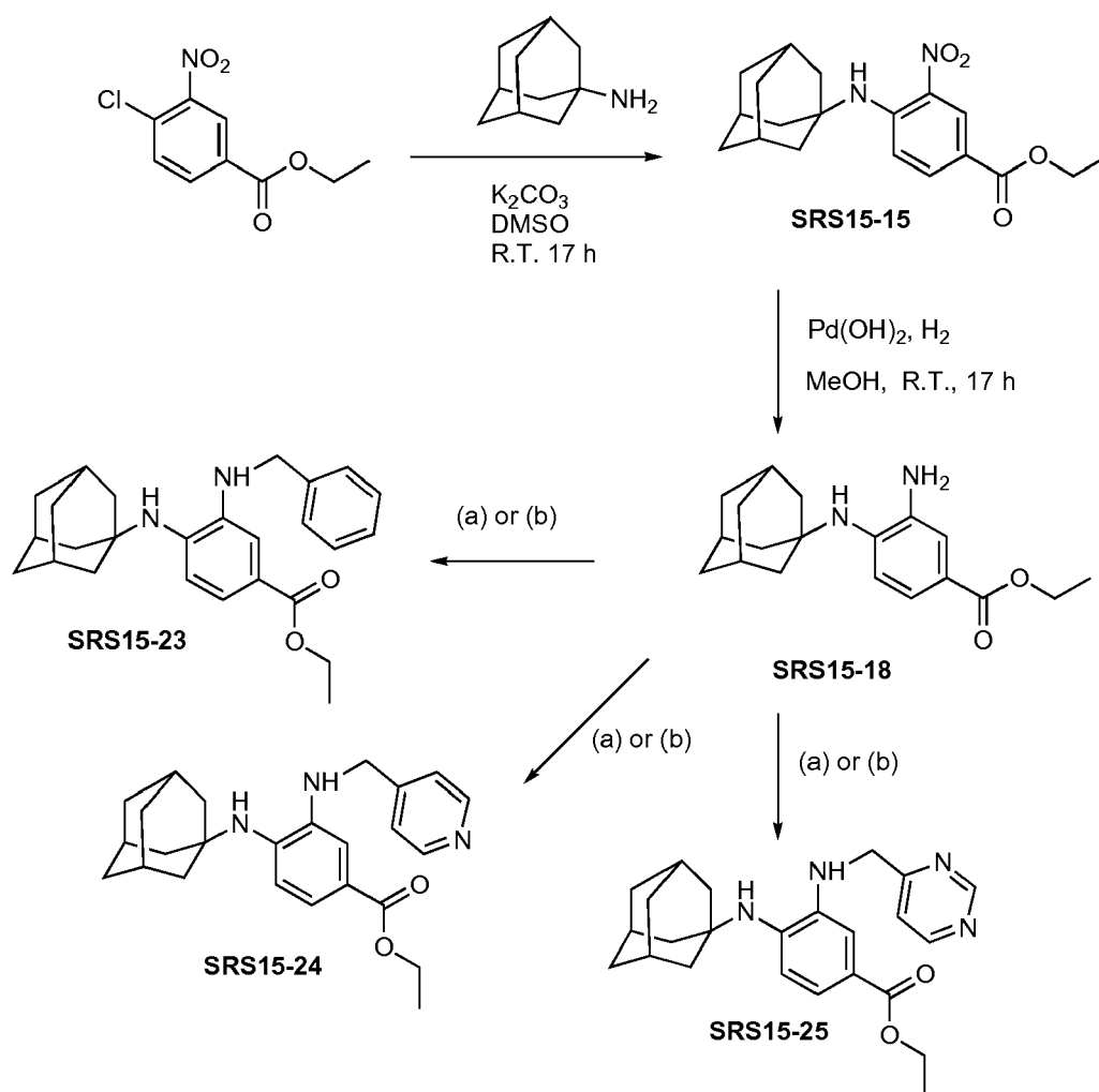
Scheme 1. Synthesis of Ferrostation analogs SRS15-18, SRS15-23, SRS15-24, SRS15-25. (a) alkylation reaction: arylhalide, DIPEA, THF, 60 °C, 17 h. (b) reductive amination reaction: arylaldehyde, \text{NaBH}(\text{OAc})_3 , molecular sieve (4 Å), DCE, R.T. to 80 °C, 17 h.
