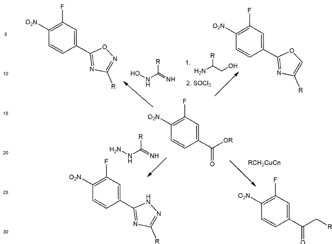
Scheme 8: Synthesis of Fer-1 analogs containing ester bioisosters
