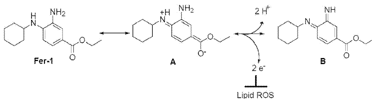
Scheme 6: Fer-1 as a reducing agent: release of 2 protons and 2 electrons results in a formation of ethyl 4-(cyclohexylimino)-3-iminocyclohexa-1,5-dienecarboxylate intermediate B.
