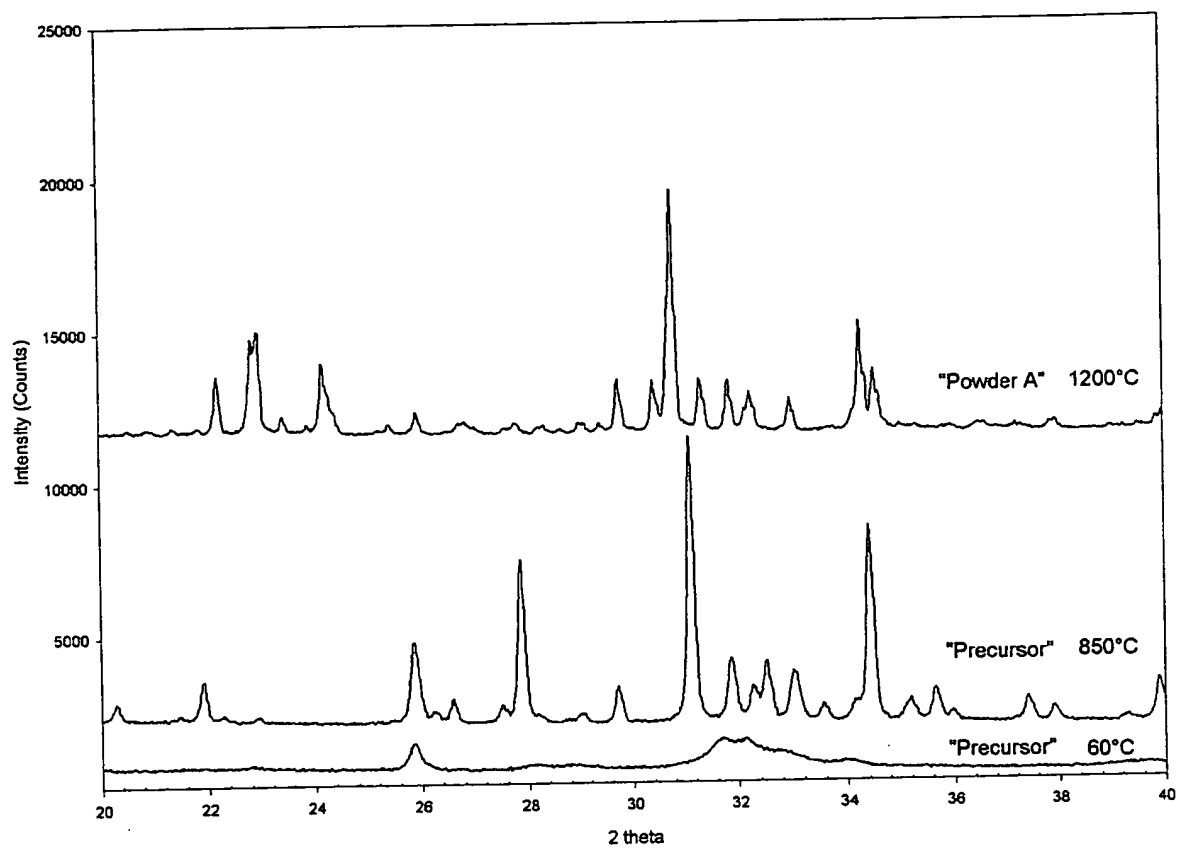
Fig. 1 Powder XRD traces of the precursors and the powder obtained in Example-1
