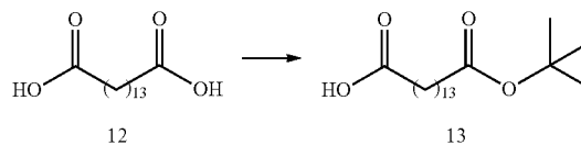
15-(tert-butoxy)-15-oxopentadecanoic Acid, 13
