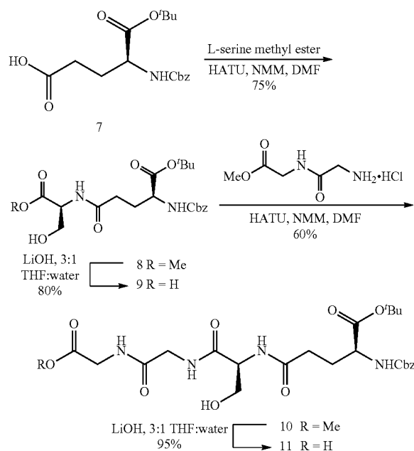
(S)-tert-butyl 2-(((benzyloxy)carbonyl)amino)-5-(((S)-3-hydroxy-1-methoxy-1-oxopropan-2-yl)amino)-5-oxopentanoate, 8
