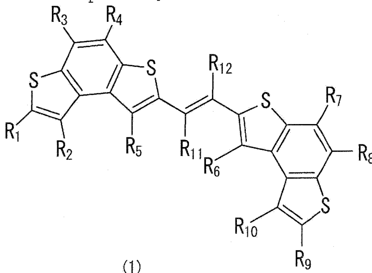
[Chemical Compound 1]
