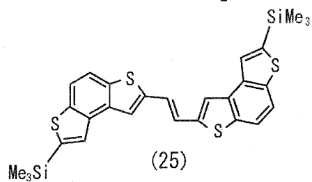
[Chemical Compound 5]
