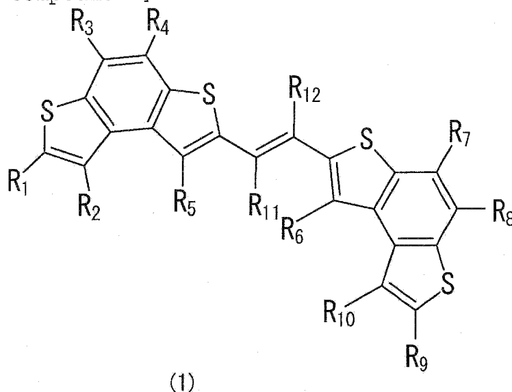
[Chemical Compound 7]
