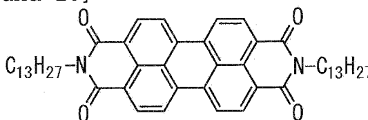
(4) (PTCDI-C13)
