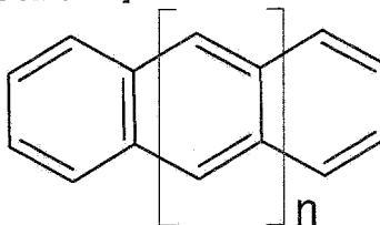
[Chemical Compound 1]
