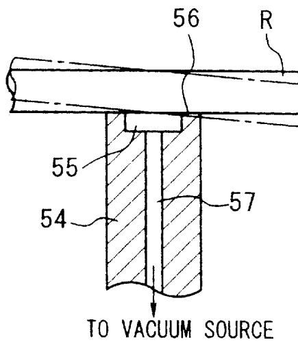
FIG. 10C PRIOR ART
