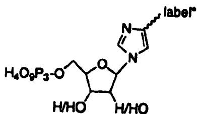
Imidazole
