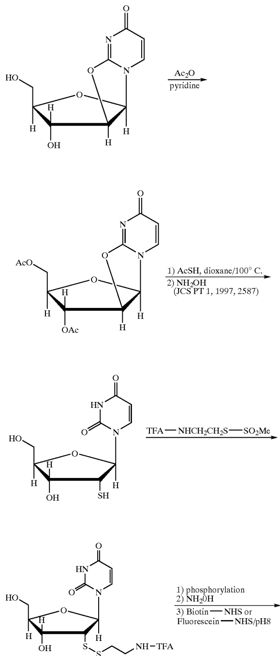
Scheme 10.
