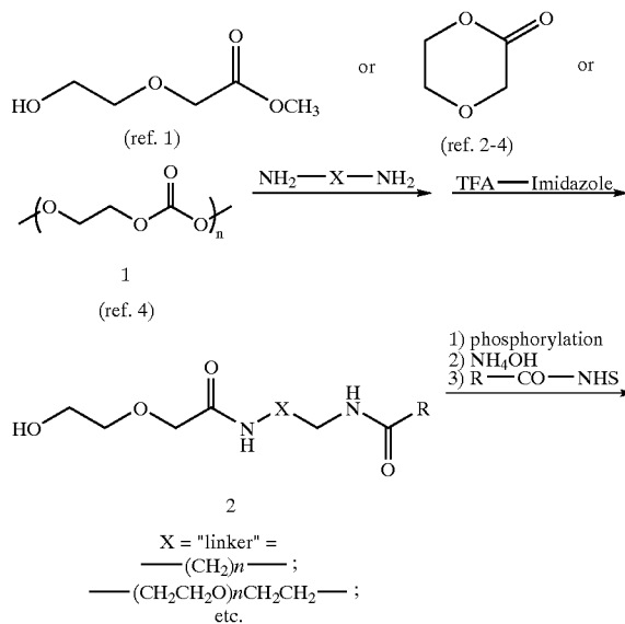
Scheme 7
