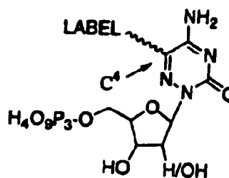
C/dC analogs
