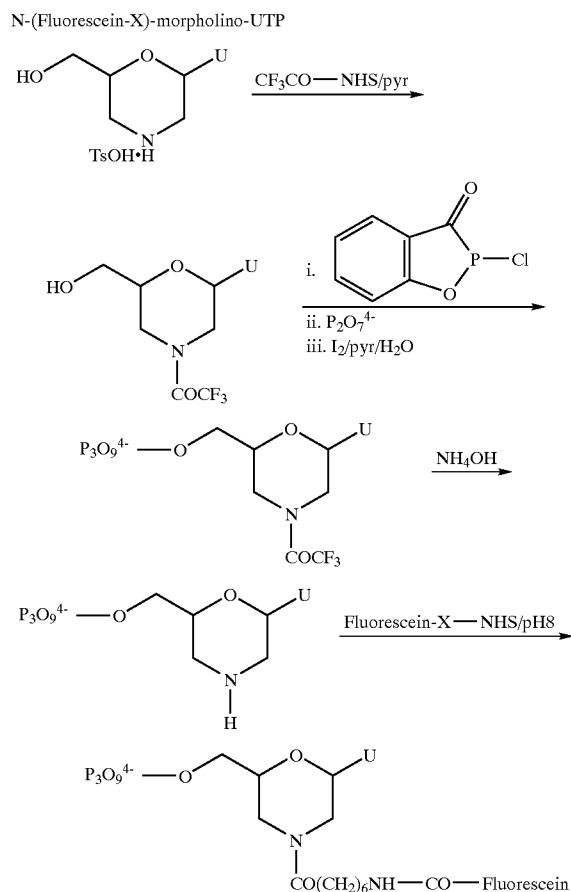
Scheme 5
