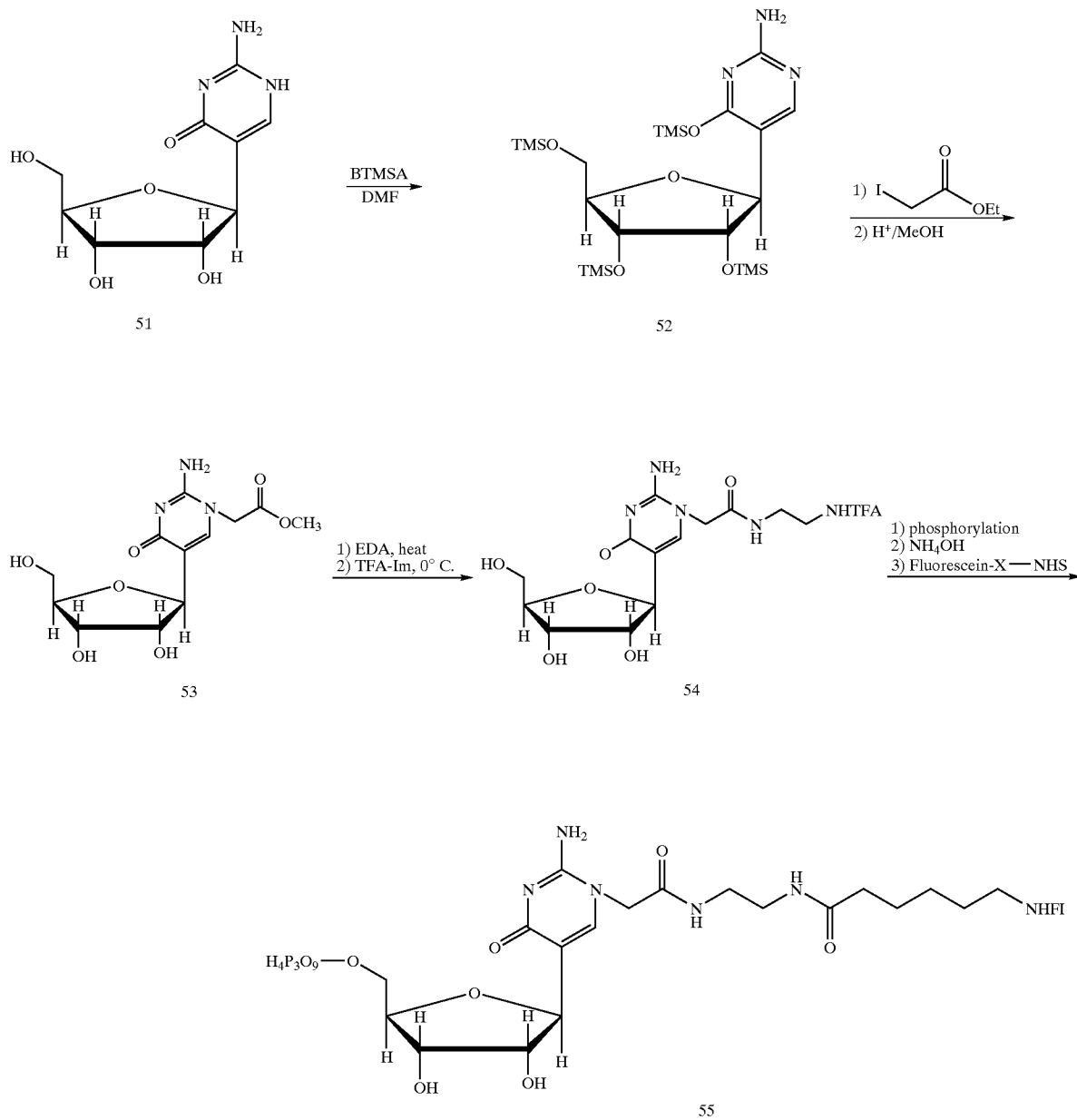
Scheme 2
