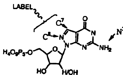
G/dG analogs
