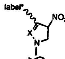
nitro-pyrrole/pyrazole
