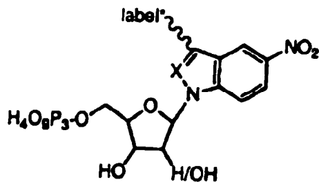
nitro-indole/indazole
