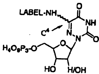
U/T analogs
