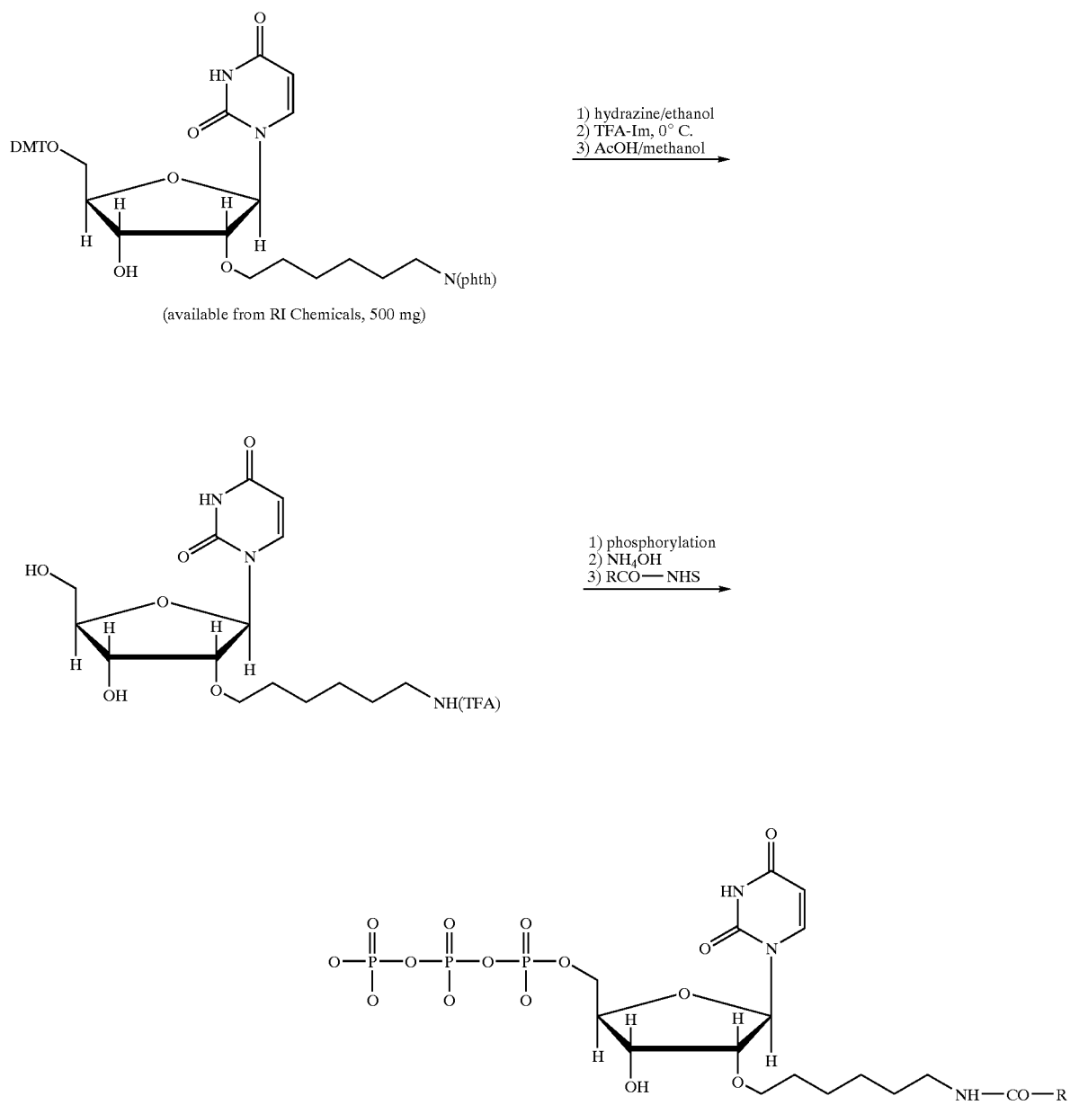
Scheme 9.
