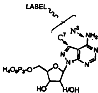
A/dA analogs
