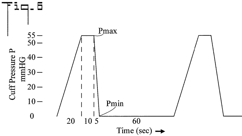
PRESSURE APPLICATION MODE 1
