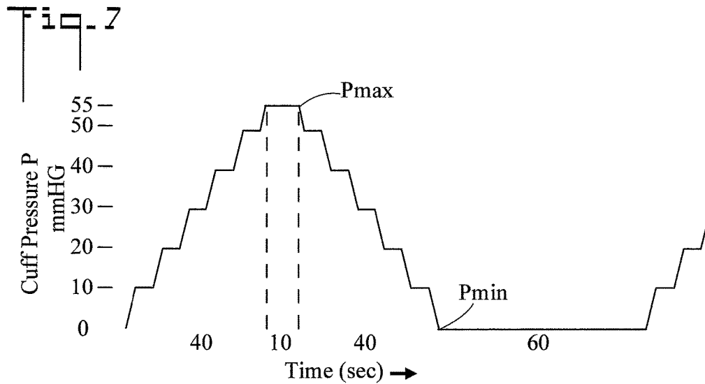
PRESSURE APPLICATION MODE 2
