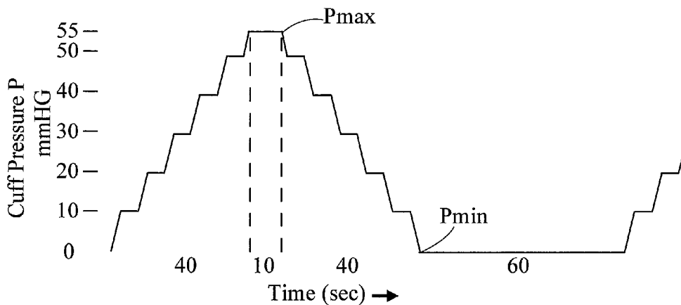
PRESSURE APPLICATION MODE 2
