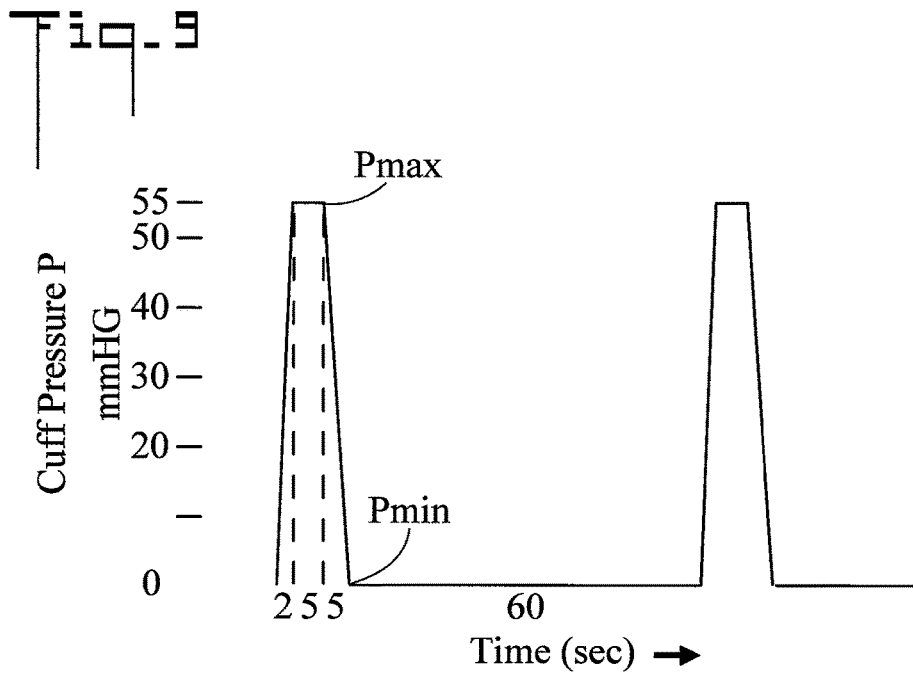
PRESSURE APPLICATION MODE 4
