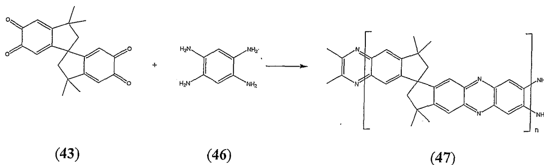
Reaction scheme D
