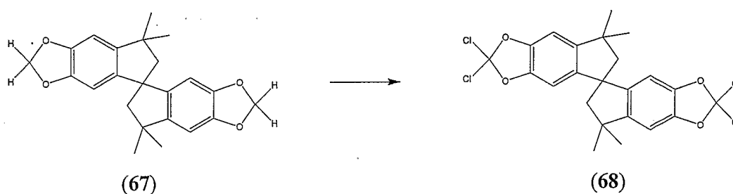
Reaction scheme H
