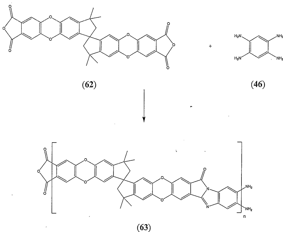
Reaction scheme F
