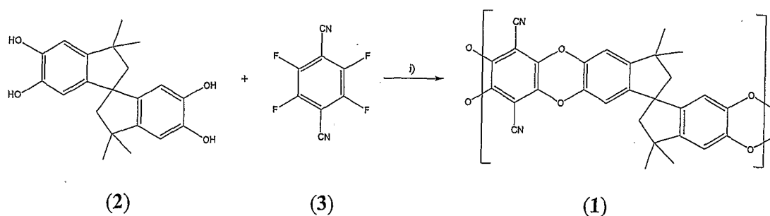
Reaction scheme A: synthesis of polydioxane A (1); i) K_2CO_3 , DMF, 50^\circ C
