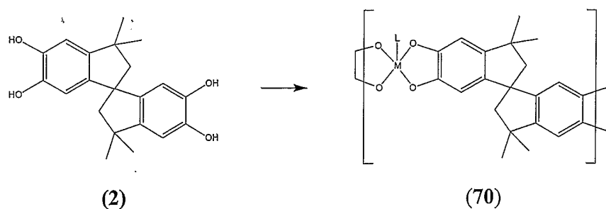
Reaction scheme J
