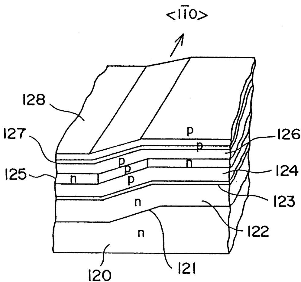
FIG. 4 (RELATED ART)
