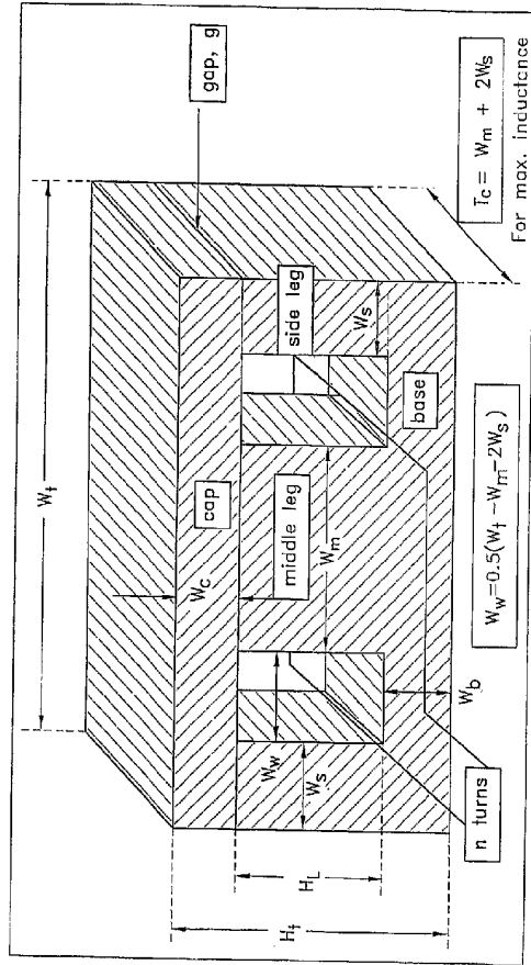
Ferromagnetic E core with a matching ferromagnetic cap
