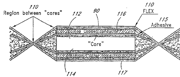
Side view showing top & bottom FLEX laminated to "core" in a panel of 70 "cores"
