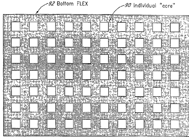
Array of 70 cores laminated onto a large panel of FLEX (top FLEX removed to show the individual cores)
