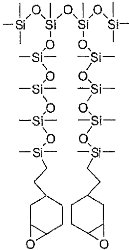
epoxy-Si-12
