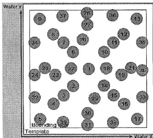
Resist drop layout
