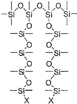
Functionalized Si-12
