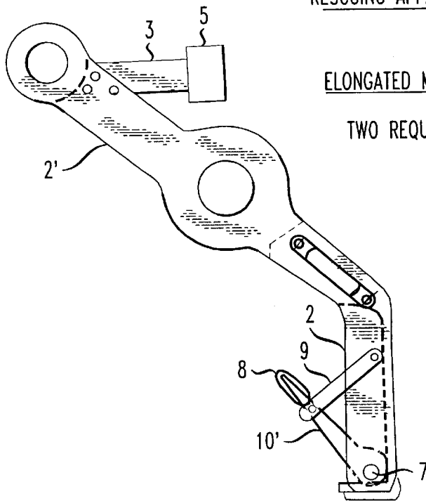
CARGO RETRIEVAL AND RESCUING APPARATUS
