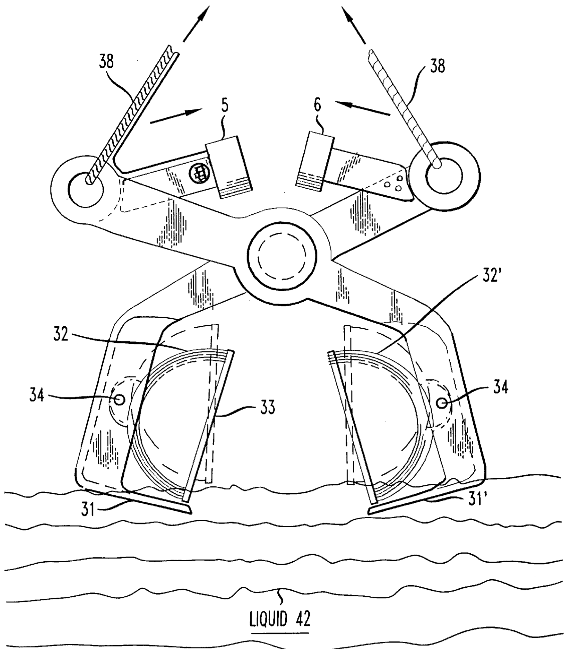
PERSONNEL RESCUING APPARATUS, LOWER PORTIONS SEPARATED
