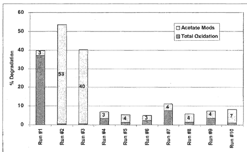
Figure 16. HPLC Degradation Profile (T=1M, 25C)
