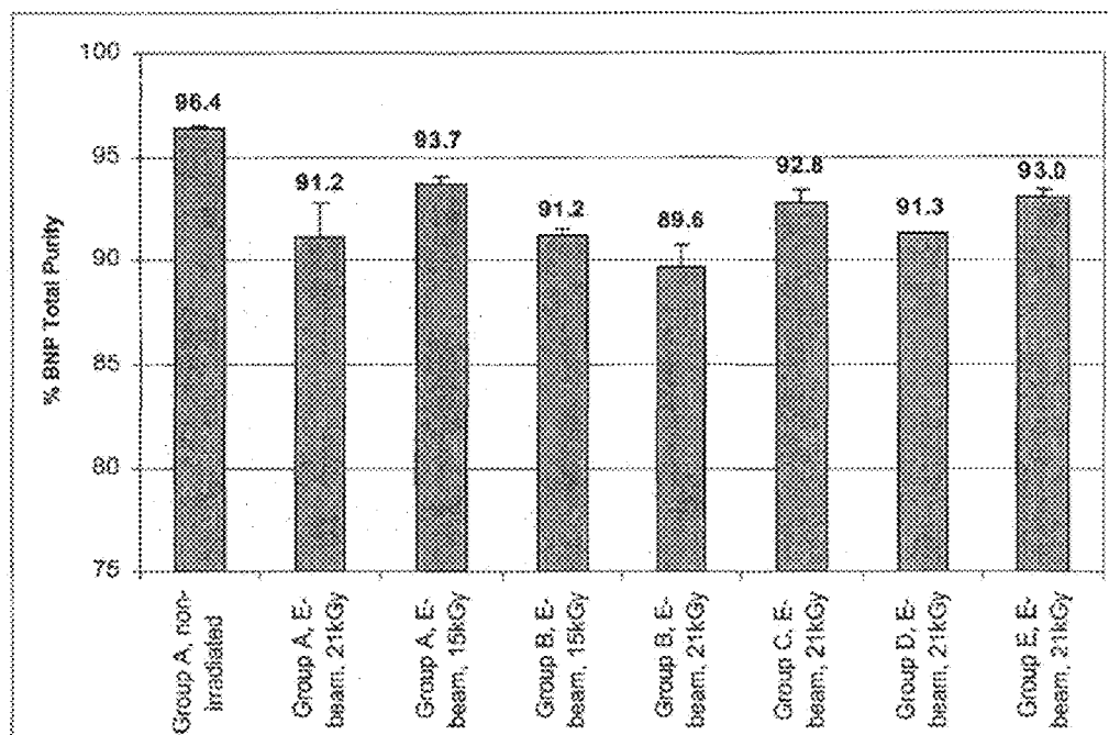
Figure 9. BNP Degradation Profile by HPLC at T=0
