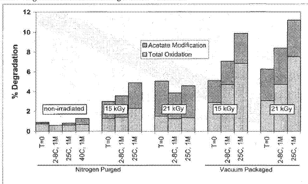
Figure 12. Degradation Profile following E-Beam Treatment
