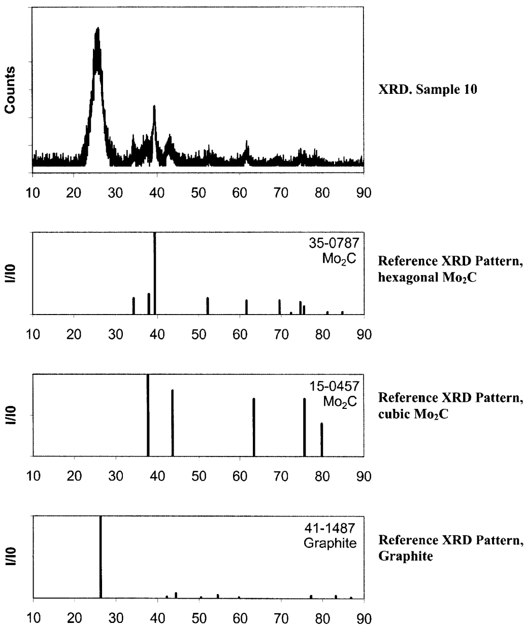
FIG. 3A XRD and HRTEM of CARBIDE NANOPARTICLES SUPPORTED ON CARBON NANOTUBES
