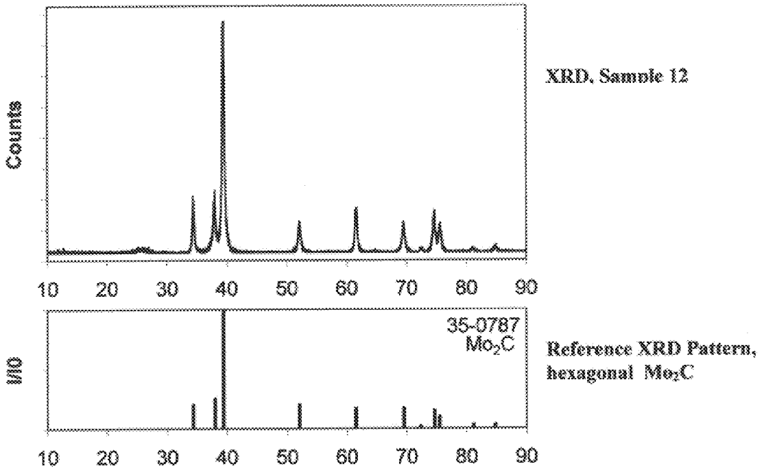
FIG. 2A XRD and HRTEM of CARBIDE NANORODS
