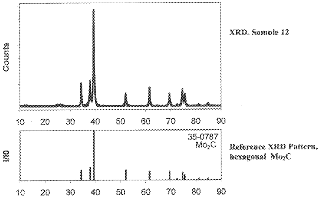
FIG. 1A XRD and SEM of CARBON NANORODS
