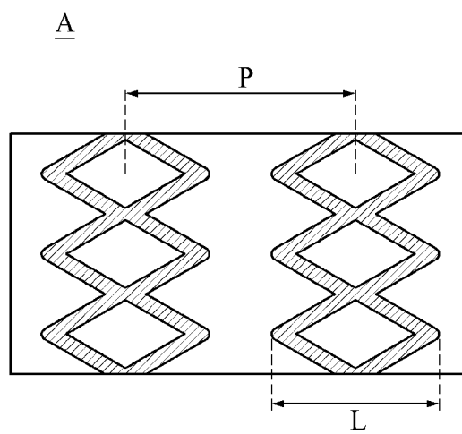
FIG. 2 (RELATED ART)
