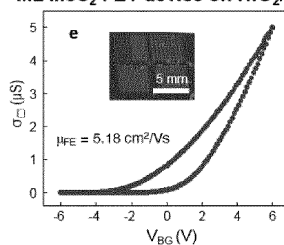
ML MoS 2 FET device on HfO 2 /Si
