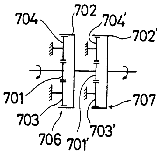
Fig. 9 (PRIOR ART)
