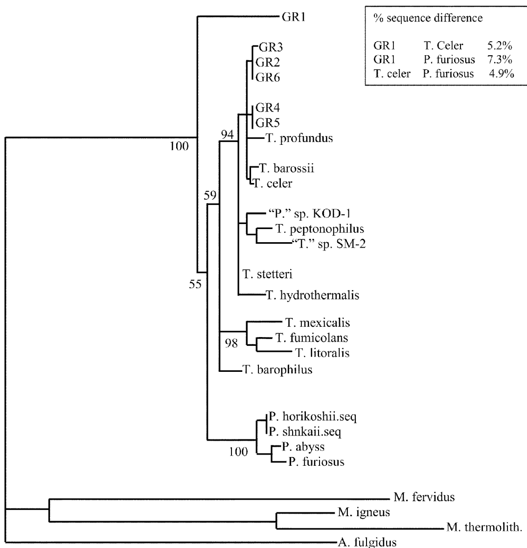
Neighbor-joining tree for Thermococcales
