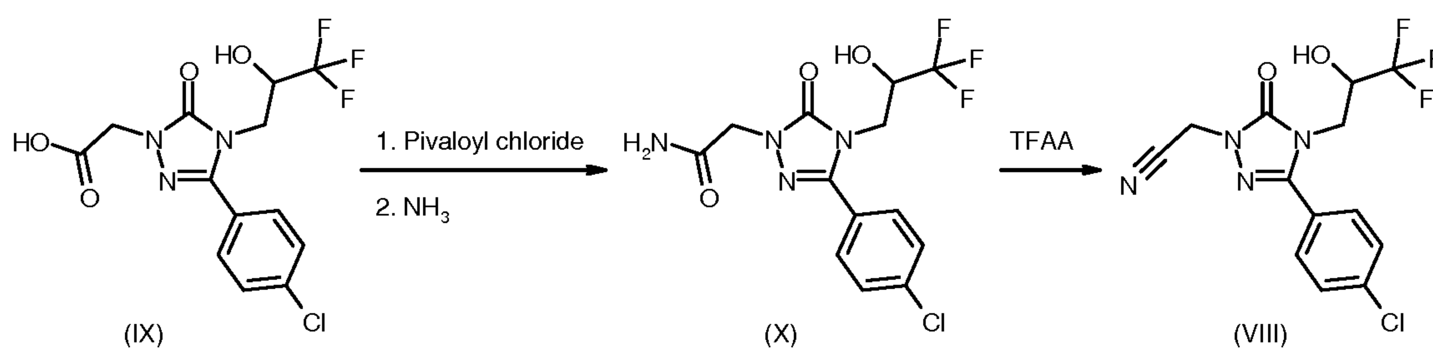
Scheme 2
