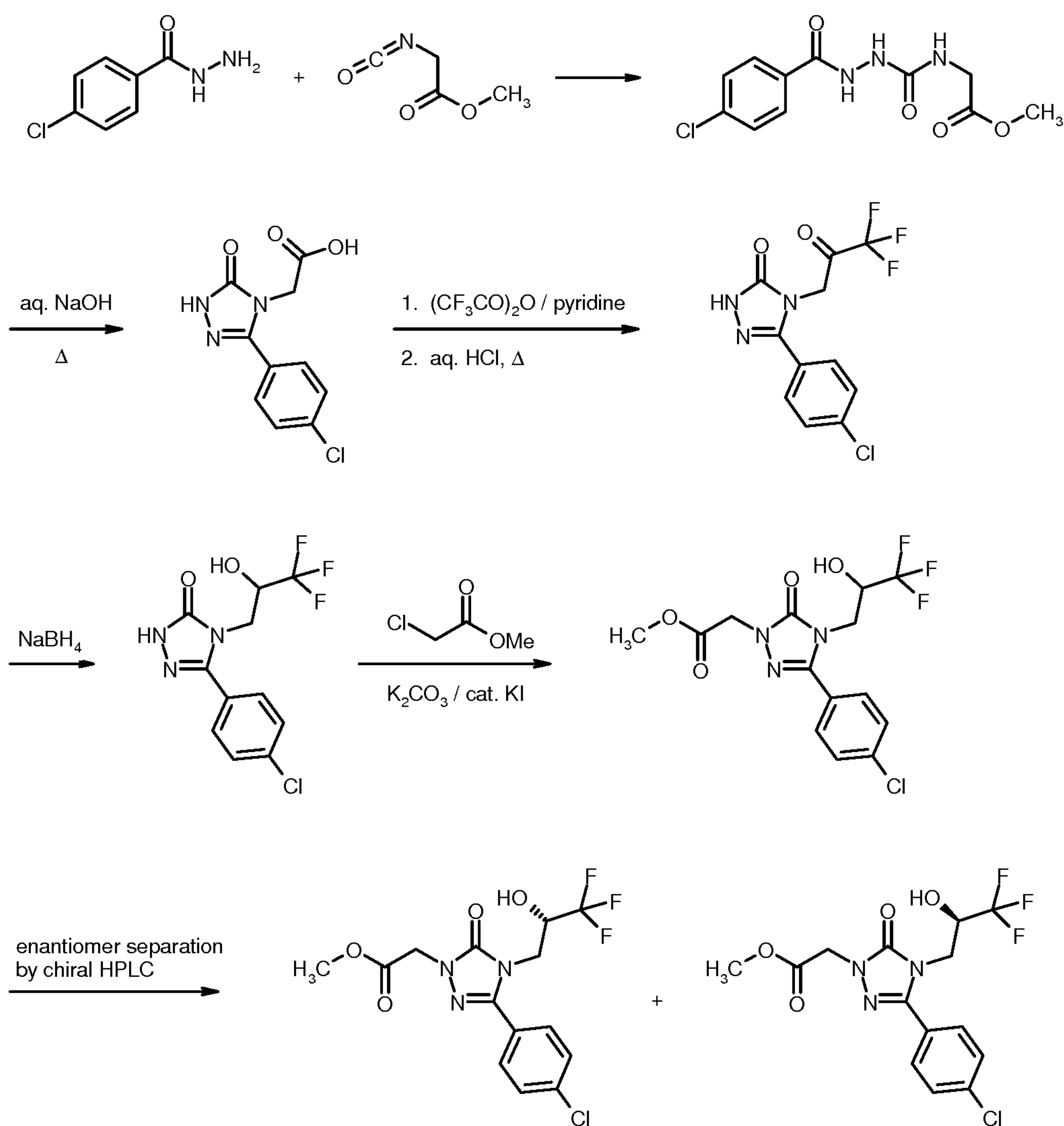
Scheme 3
