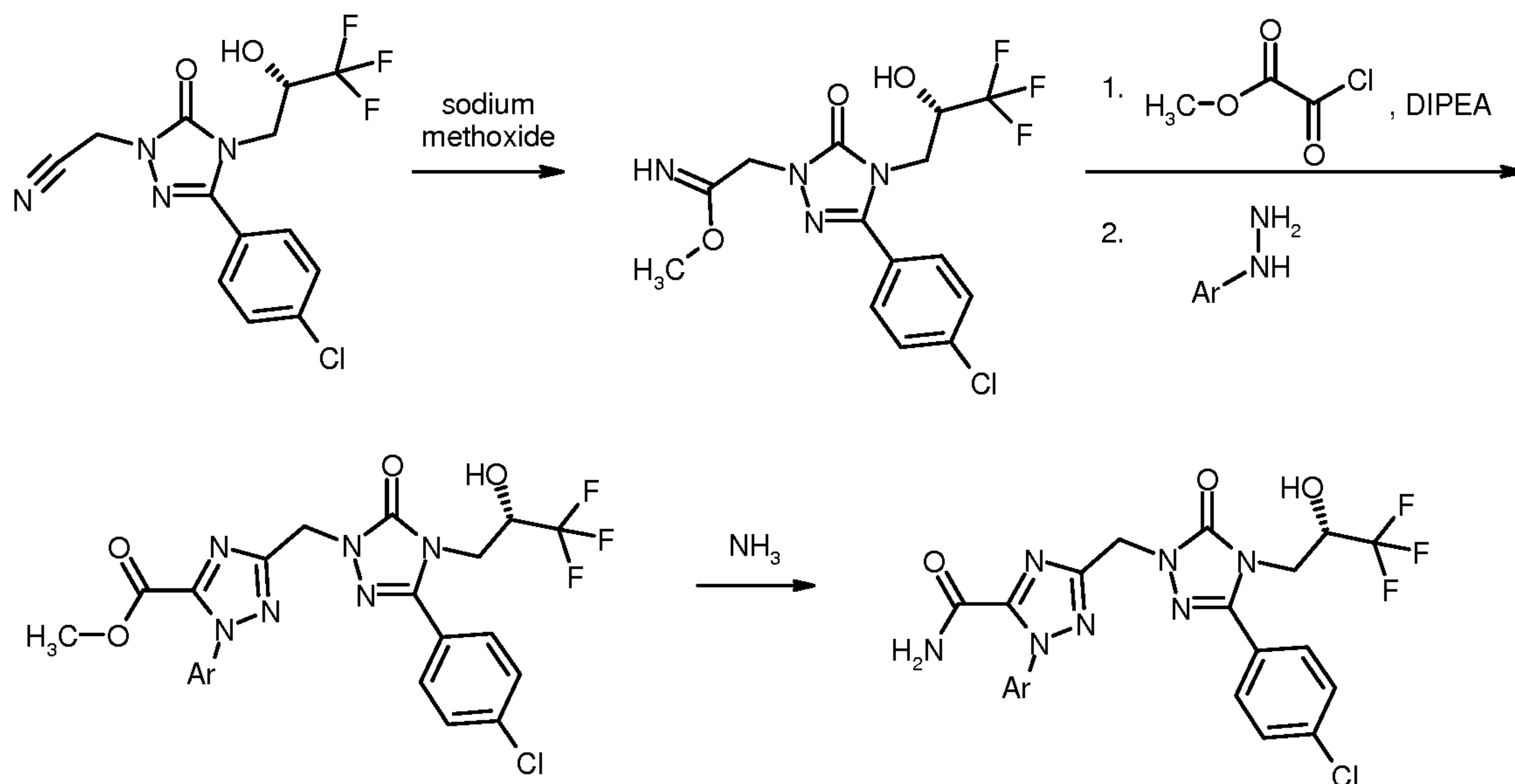
Scheme 7
