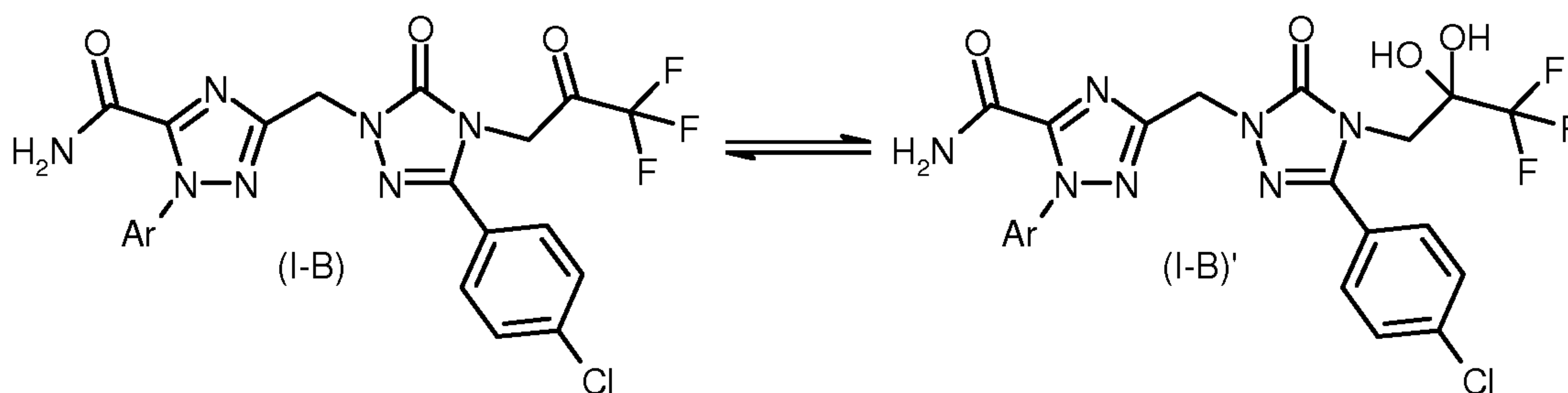
Scheme 1
