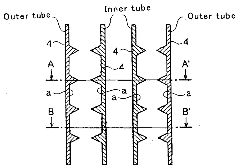
A-A' Cross section
