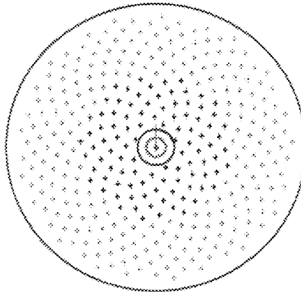
1.0 mm dia 344 holes 5" disc 3.7% removed area
