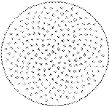
2.65 mm dia holes 5" disc 10.8% removed area
