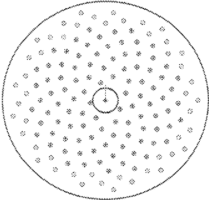
2.6 mm dia holes 5" disc 7.8% removed area
