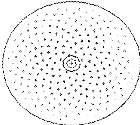
1.5 mm dia 245 holes 5" disc 5.0% removed area
