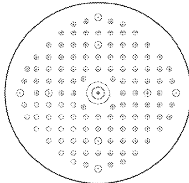
MultiAir 5" 125 holes 10.5% removed area
