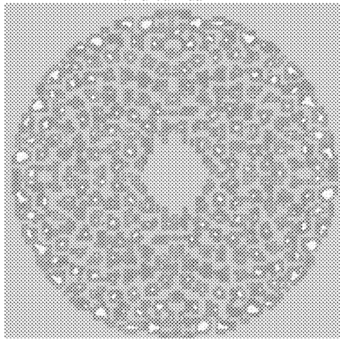
1.5 mm dia 245 holes 5" disc 5.0% removed area
