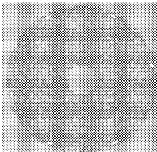
1.0 mm dia 344 holes 5" disc 3.7% removed area
