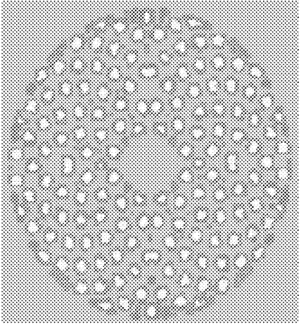
2.6 mm dia holes 5" disc 7.8% removed area
