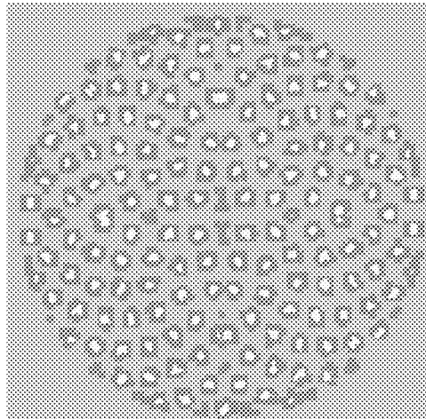
3.4 mm dia 150 holes 5" disc 10.7% removed area
