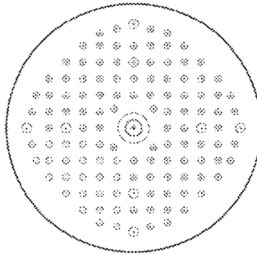
MultiAir 5" 128 holes 10.5% removed area
