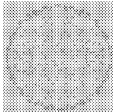
2.225 mm dia 390 holes 5" disc 10.7% removed area
