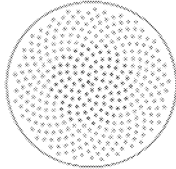
2.225 mm dia 390 holes 5" disc 10.7% removed area
