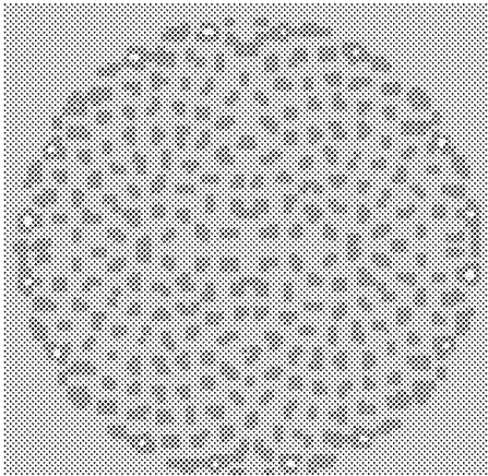
2.65 mm dia holes 5" disc 10.8% removed area
