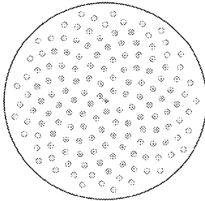
3.4 mm dia 150 holes 5" disc 10.7% removed area
