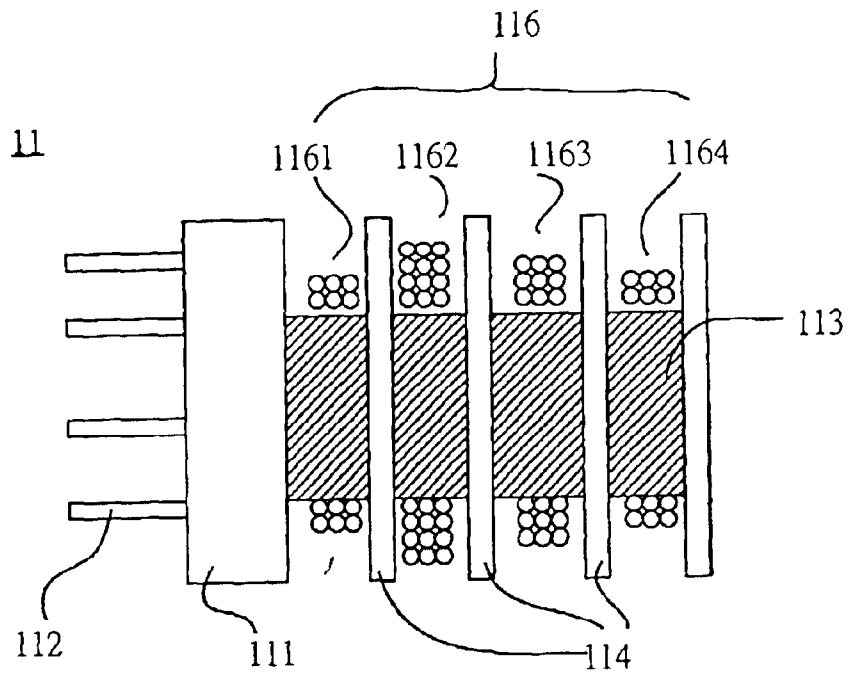
Fig.1(b)(PRIOR ART)
