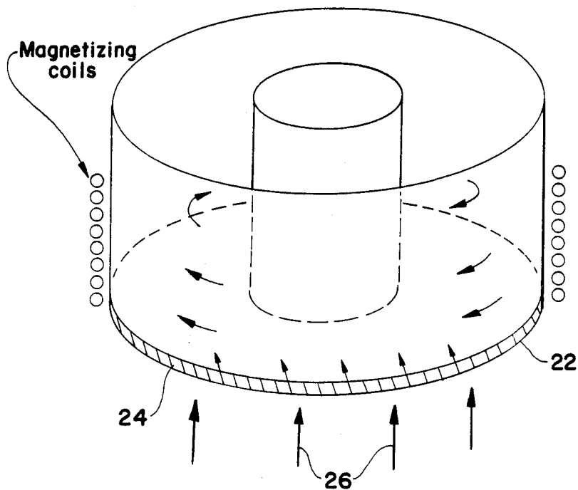
SIDE VIEW FIG. 2a
