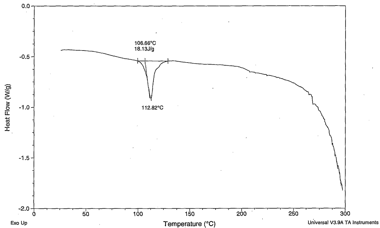
Fig. 2f DSC of Polymorph VII
