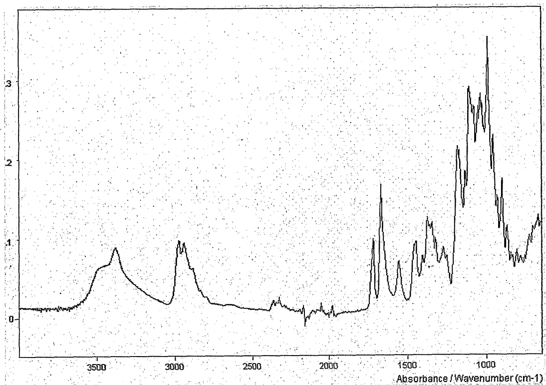
Fig.5 FT-IR spectrum for Polymorph IV
