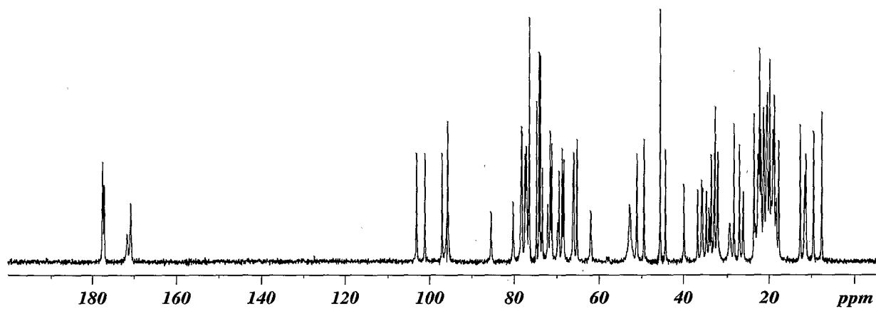
Fig.7 ^{13}\text{C} solid state NMR spectrum of Polymorph IV
