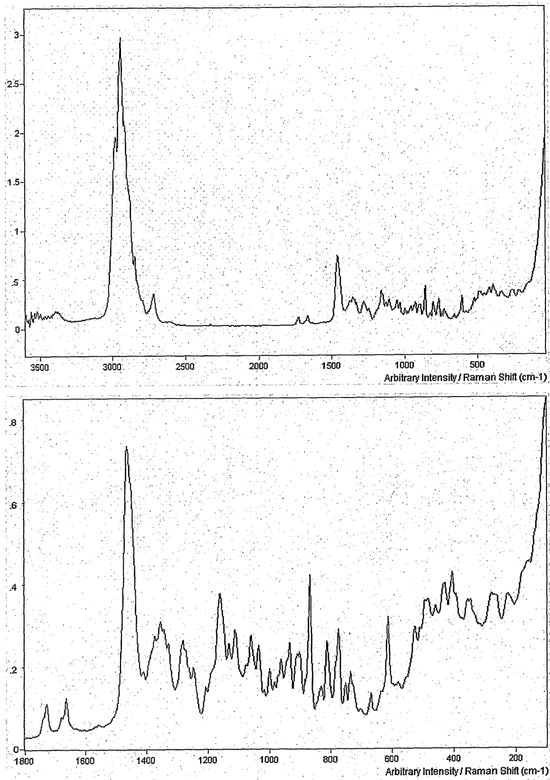
Fig.6 FT-Raman spectrum for Polymorph IV
