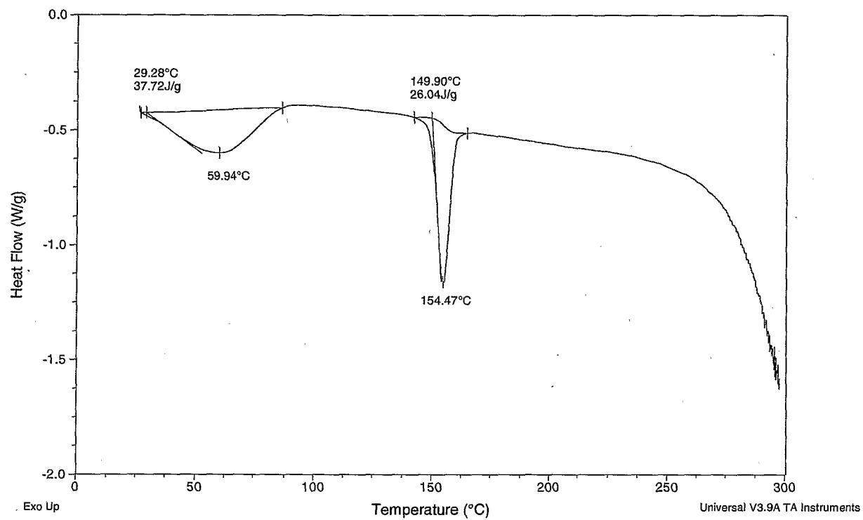
Fig. 2d DSC of Polymorph V
