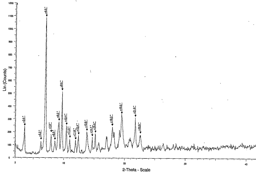
Fig. 1b XRPD of Polymorph II
