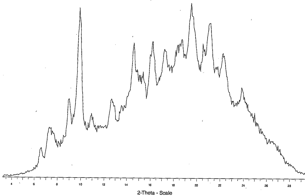
Fig. 1b XRPD of Polymorph II
