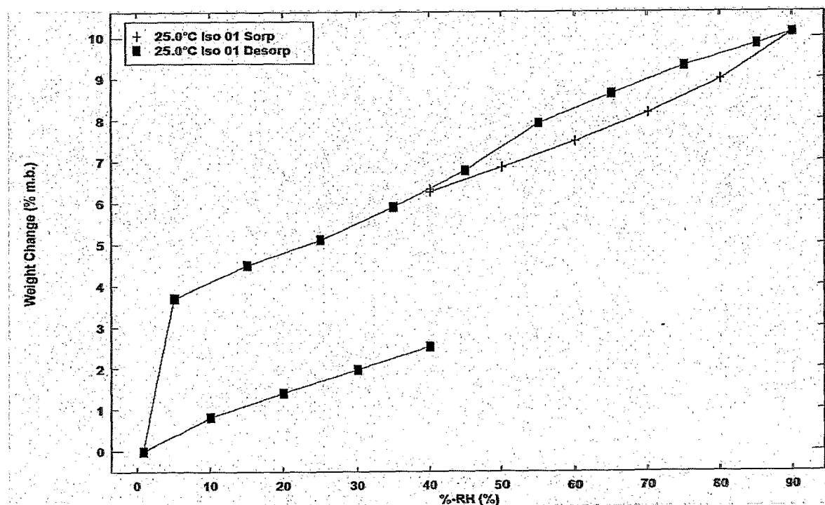
Fig. 3b GVS of Polymorph II
