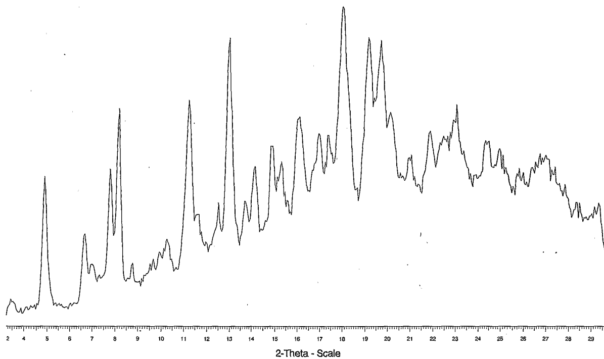
Fig. 1g XRPD of Polymorph VII
