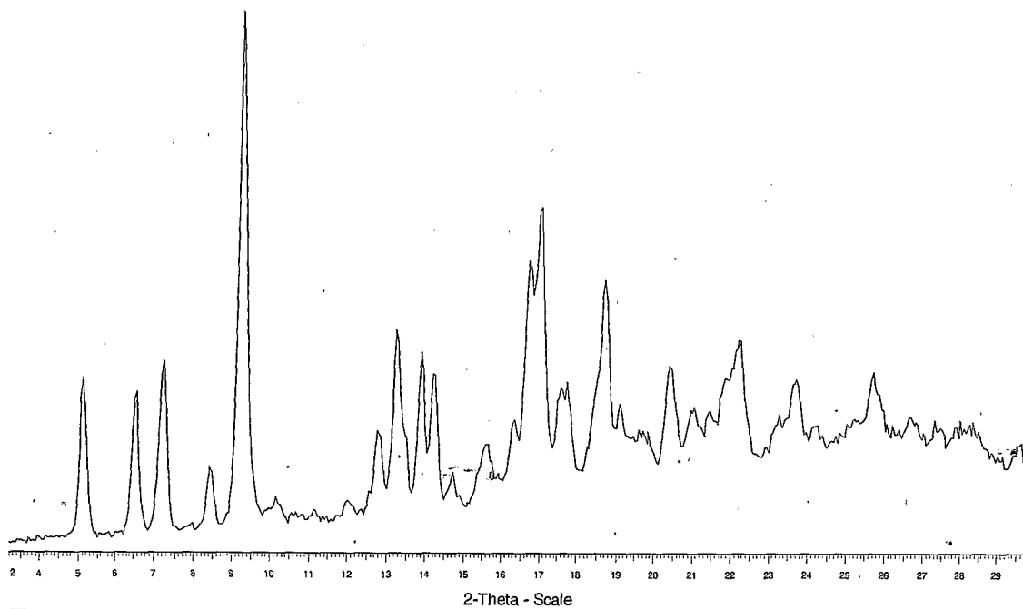
Fig. 1d XRPD of Polymorph IV
