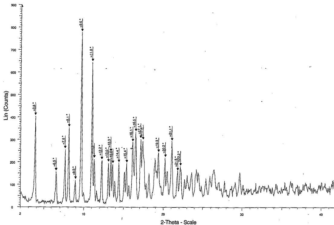
Fig. 1d XRPD of Polymorph IV
