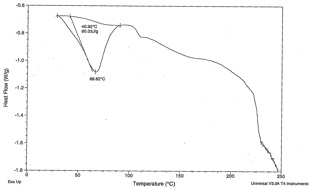
Fig. 2b DSC of Polymorph II
