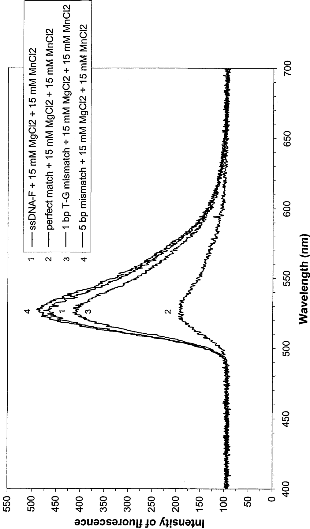
FIG. 5D. Mix of 15-mer ssDNA-F probe (4 pmole) (53% GC) and 50-mer dsDNA (0.4 pmole) in the presence of divalent cations (after 1 hr)
