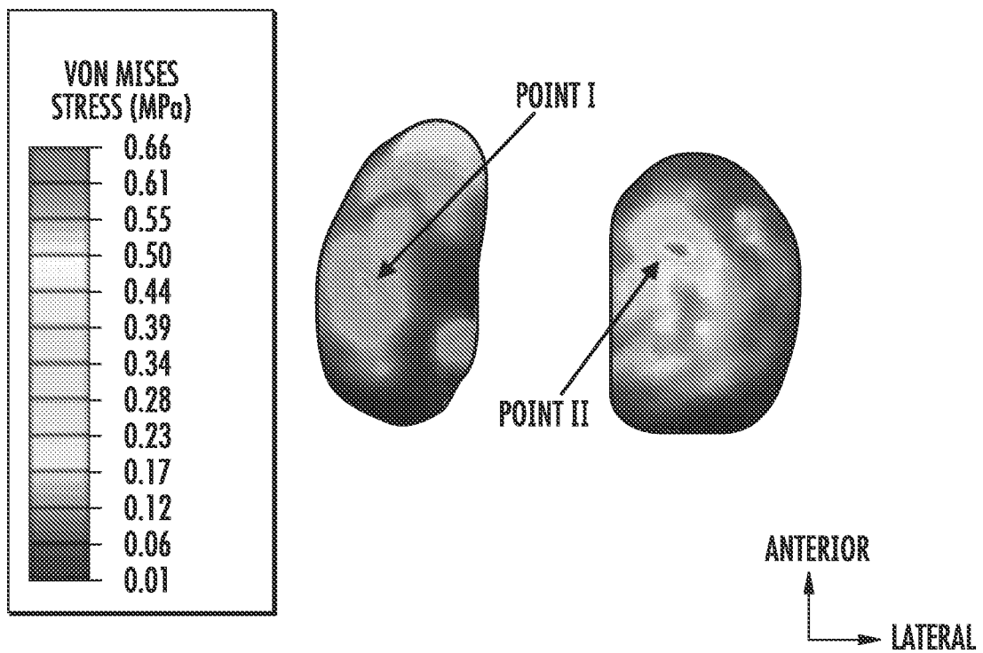
STRESS DISTRIBUTION IN TIBIAL ARTICULAR CARTILAGE
