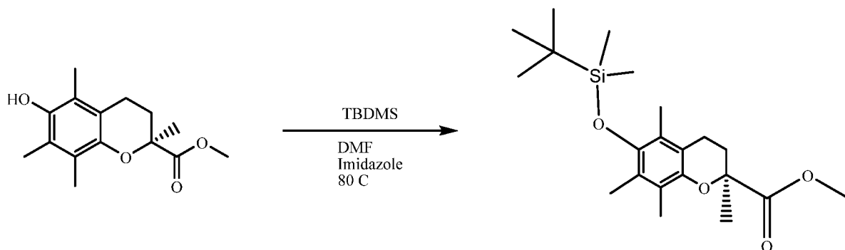
Figure 0-2: Synthesis of (S)-methyl 6-( tert -butyldimethylsilyloxy)-2,5,7,8-tetramethylchroman-2-carboxylate (S2) to protect the hydroxyl group in position 6.
