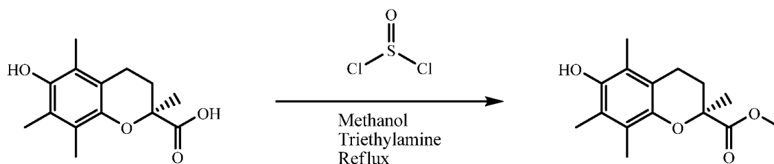
Figure 0-1: (S)-6-hydroxy-2,5,7,8-tetramethylchroman-2-carboxylic acid (Trolox) esterification
