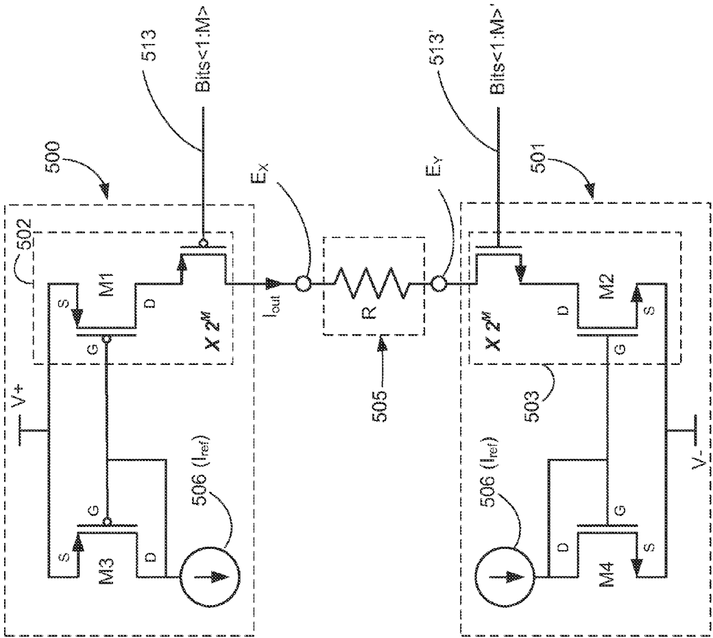
Figure 1 (prior art)
