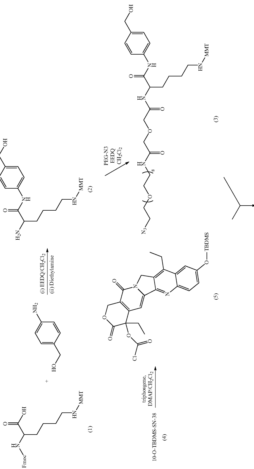
Scheme-3: Preparation of CL2A-SN-38
