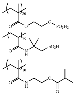
Undercoating compound (1)
