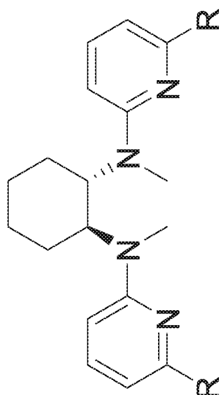
R=H; BPMCN
