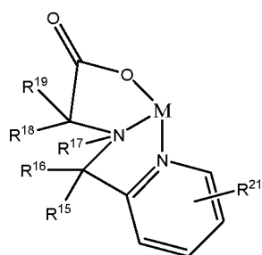
Formula VII,
