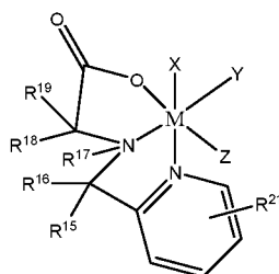
Formula VIIa,
