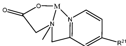
Formula IX.
