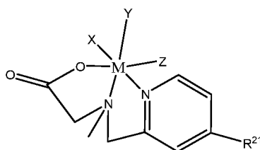
Formula IXa.
