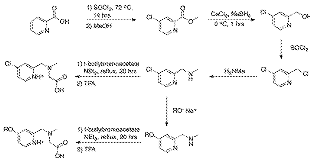
Scheme 2: Synthesis of Substituted N_2O_1 -py ligand
