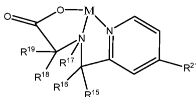
Formula VIII.
