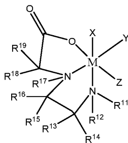
Formula Va,
