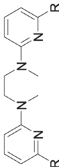
R=H; BPMEN
