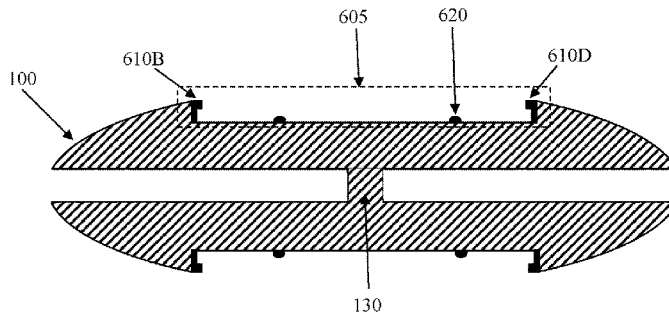
A Schematic Side-View Cut of a Latching Base in a Computerized Yo-Yo
