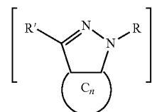
Diazoline
