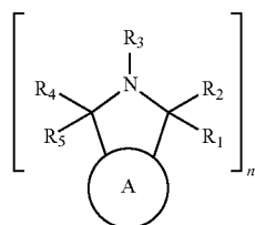
Prato Derivative
