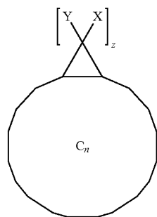
Bingel Derivative
