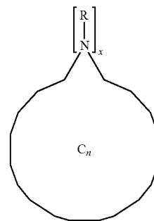
Azafulleroid
