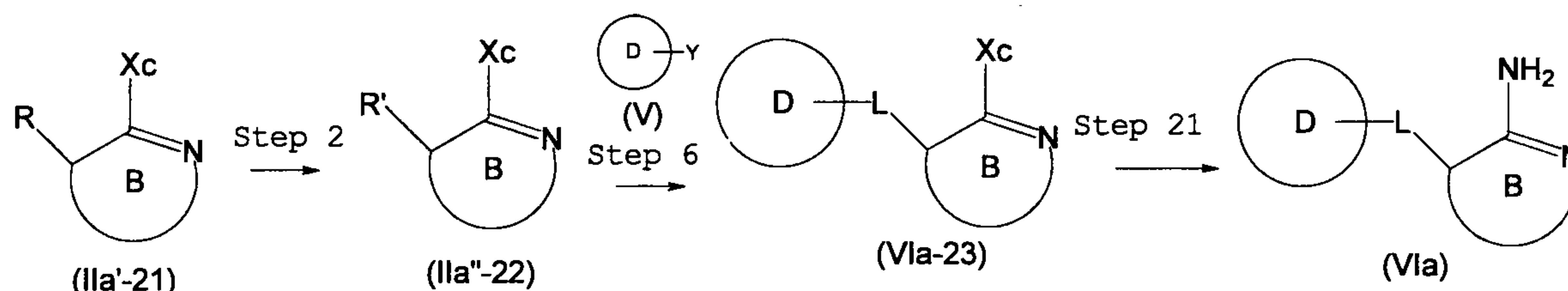
Reaction Scheme 8
