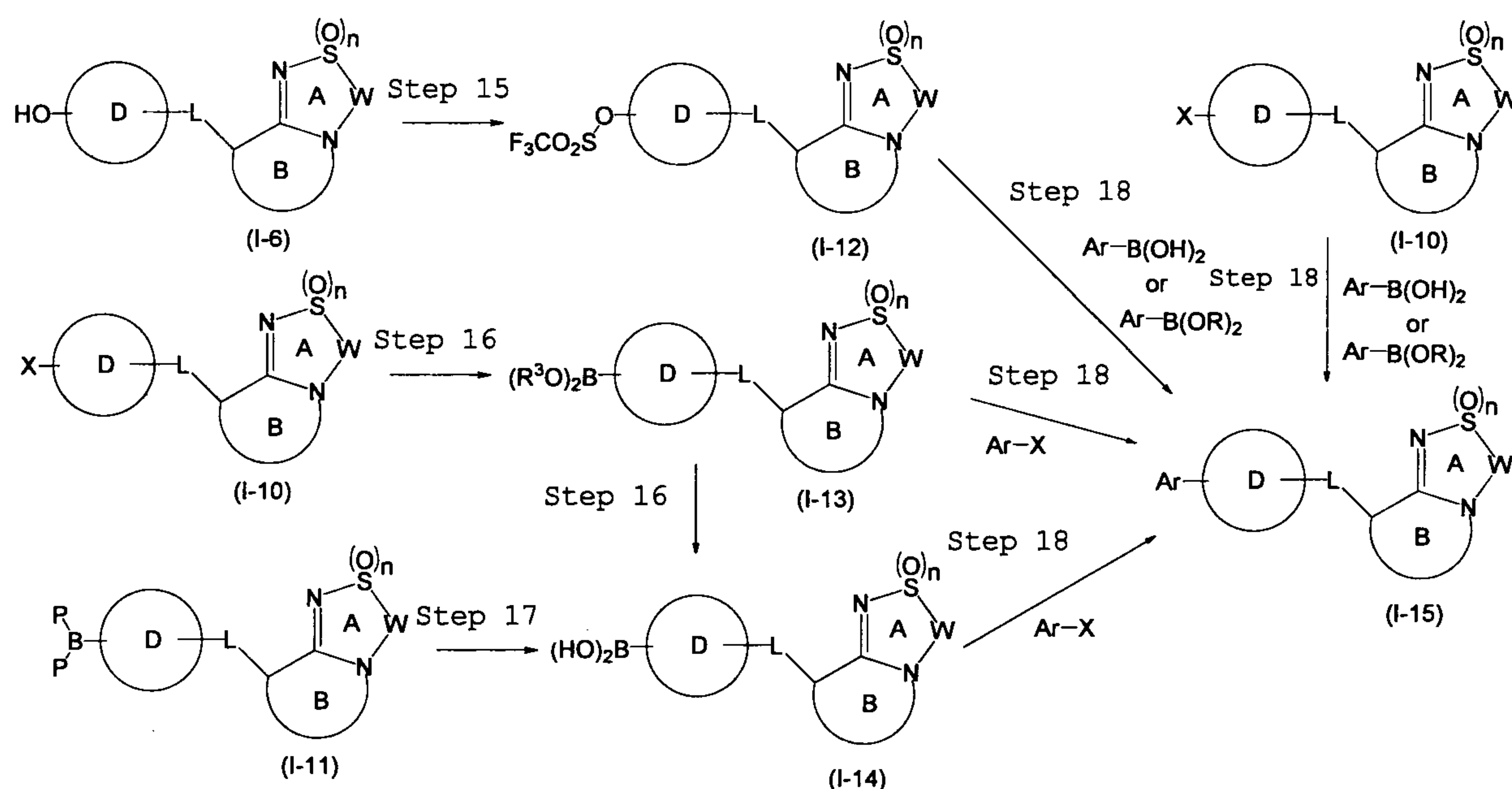
Reaction scheme 5
