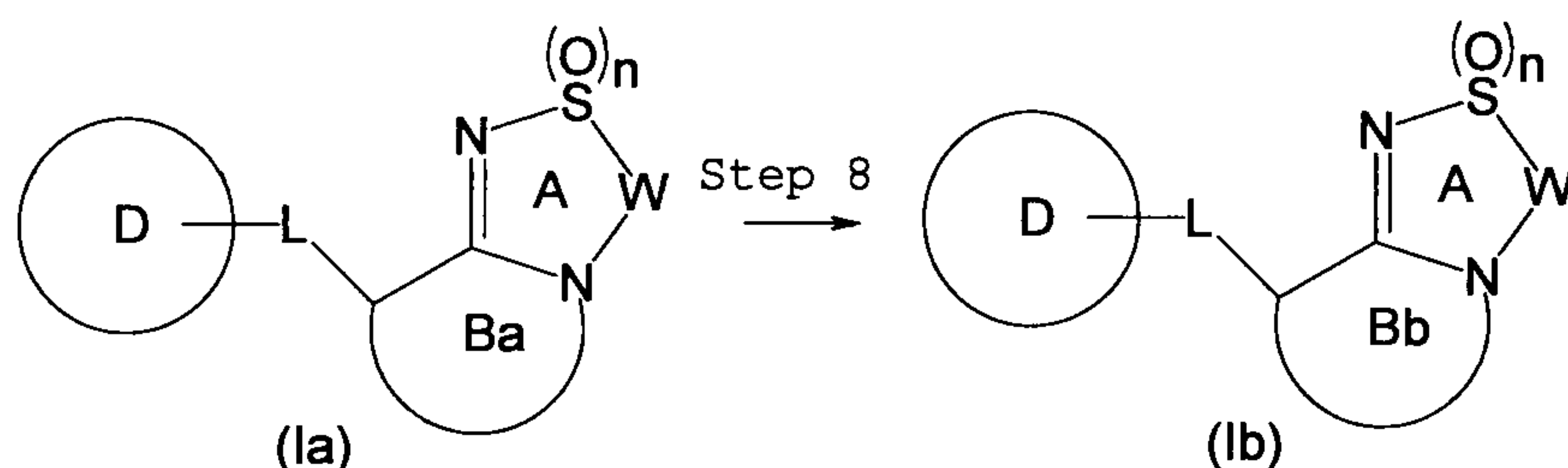
Reaction Scheme 2
