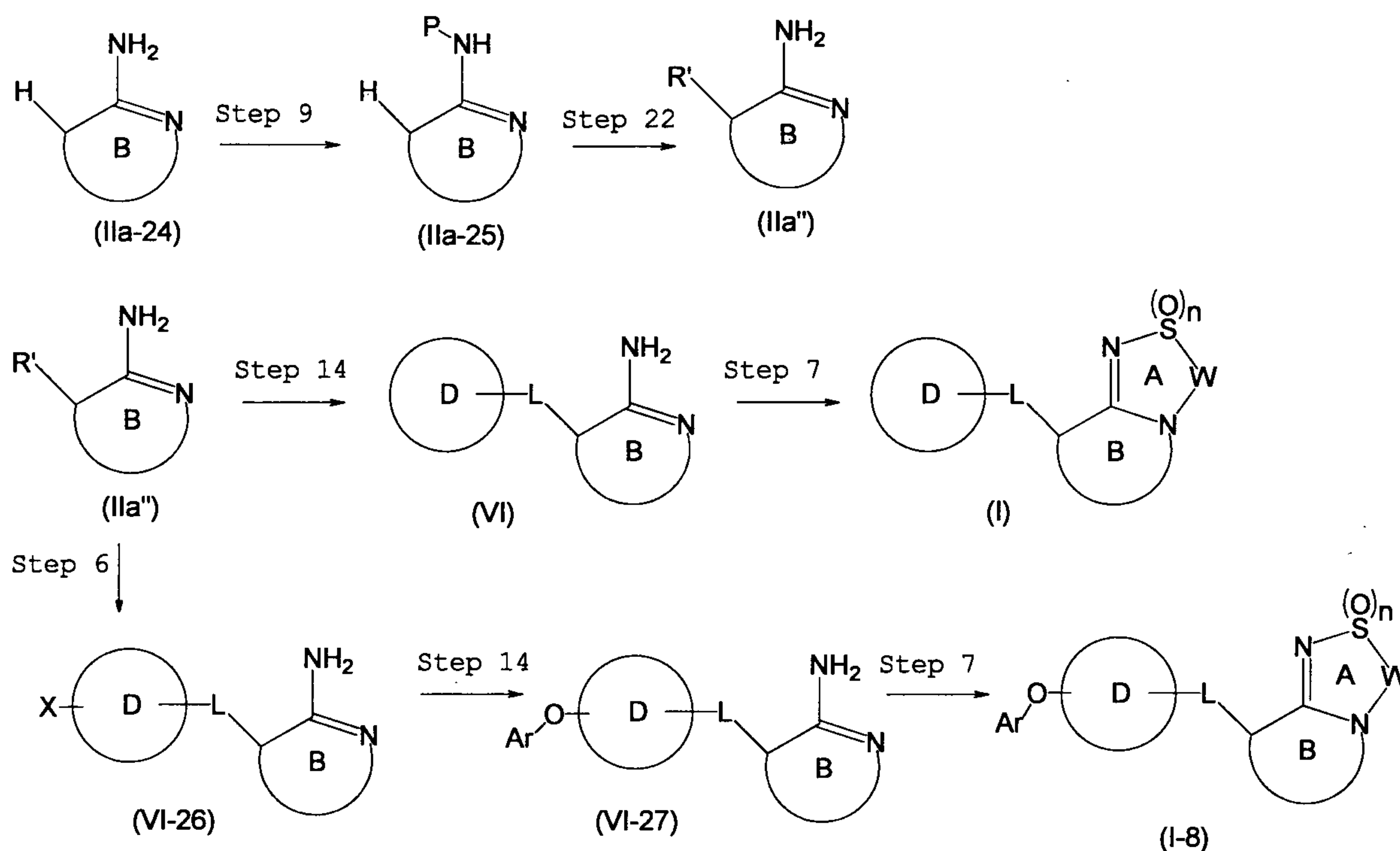
Reaction scheme 9
