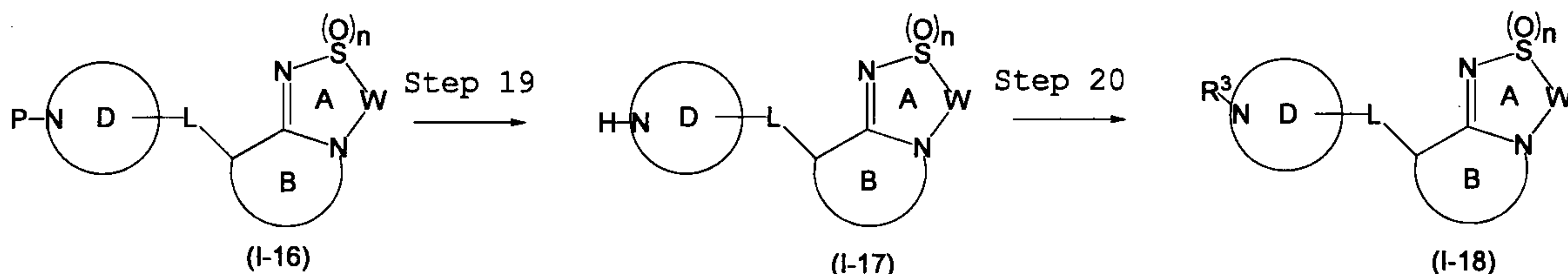
Reaction scheme 6
