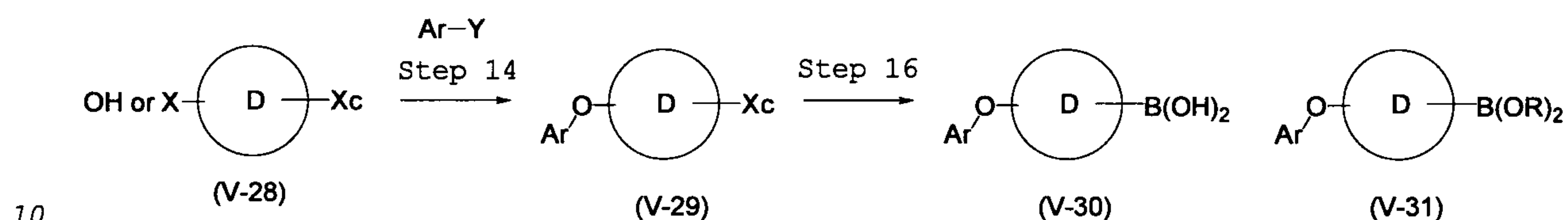
Reaction scheme 10
