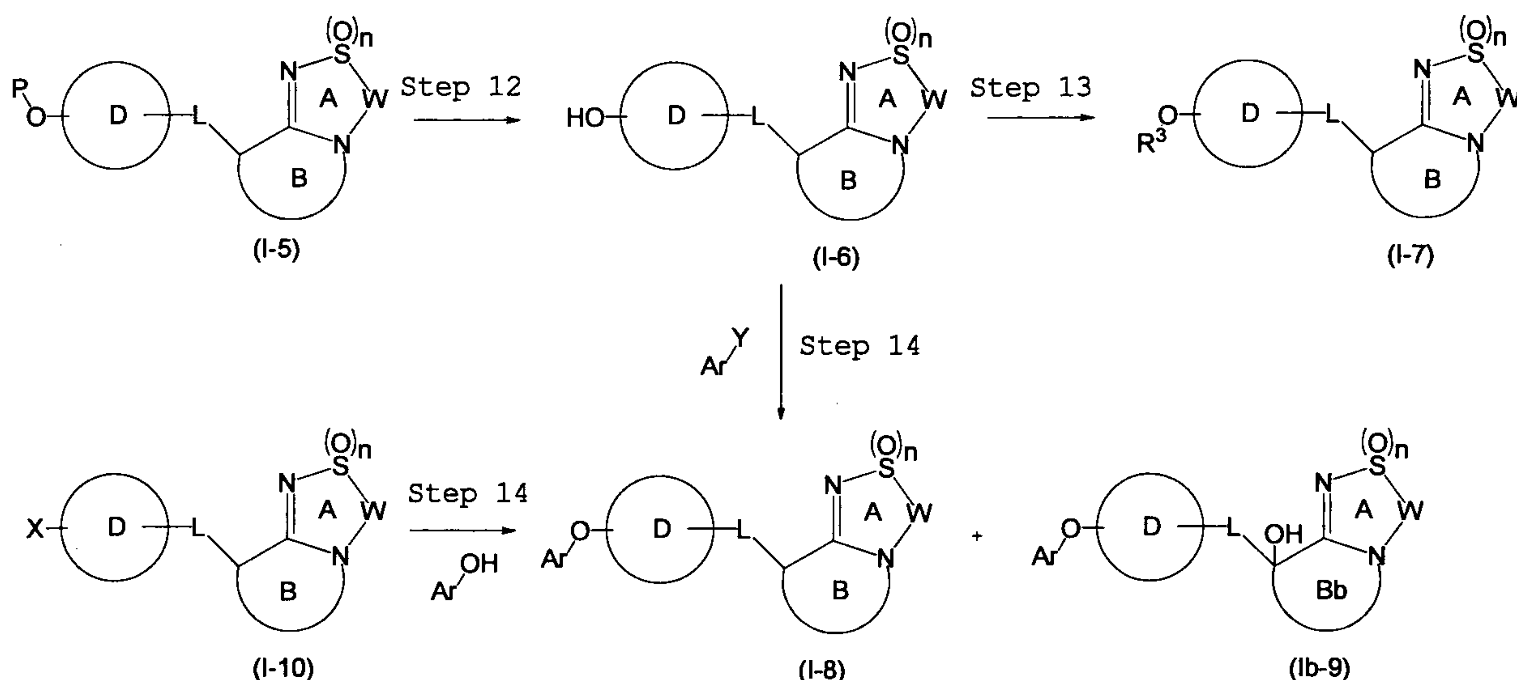
Reaction Scheme 4
