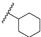
cyclohexyl
