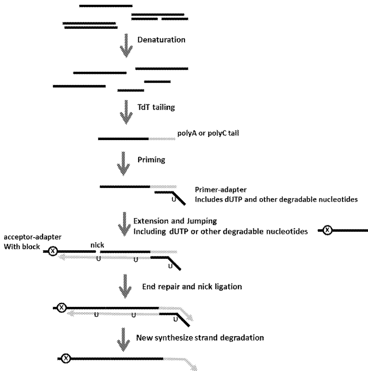
FIGURE 28 Method of generating cDNA library
