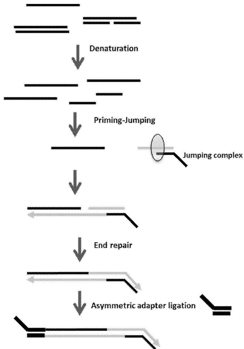
FIGURE 27 Method of generating cfDNA library
