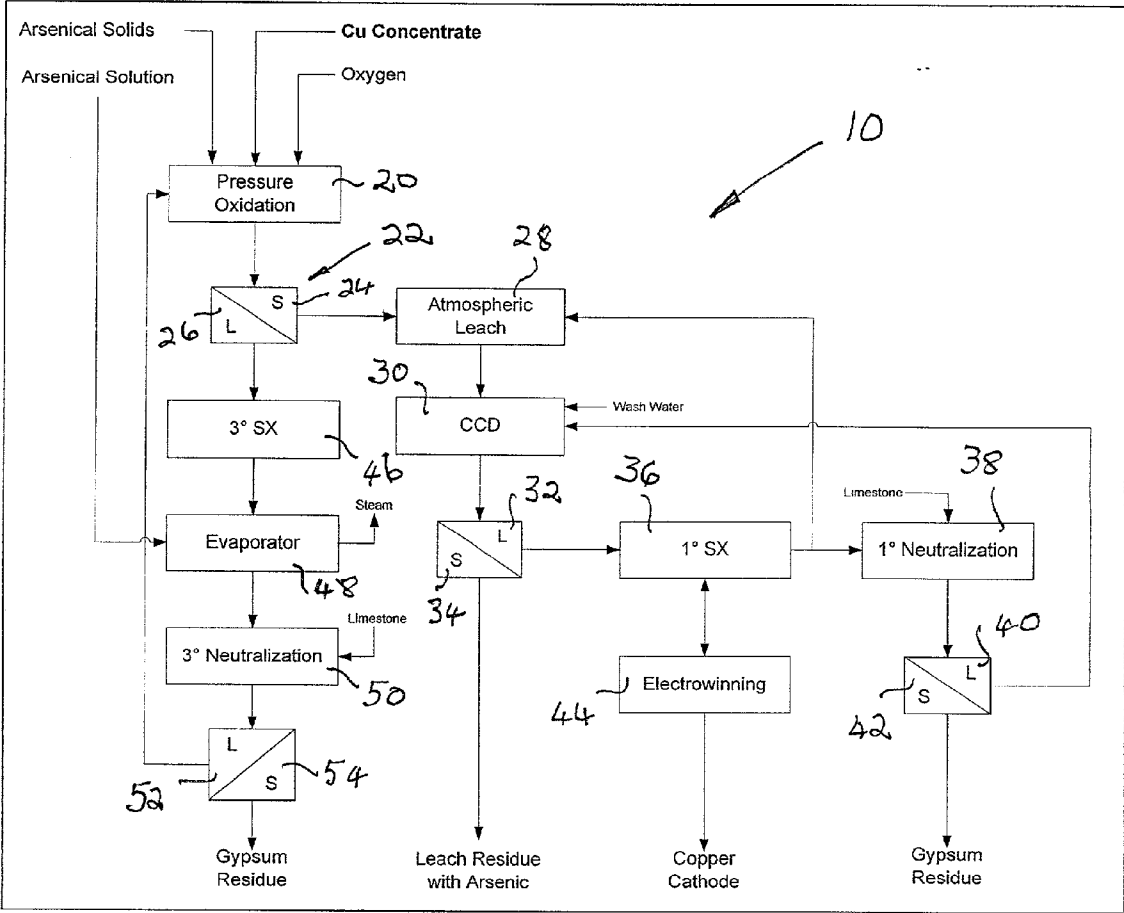
Figure 2 – CESL Refinery Process Flowsheet, including Treatment of Arsenical Byproducts from Smelter
