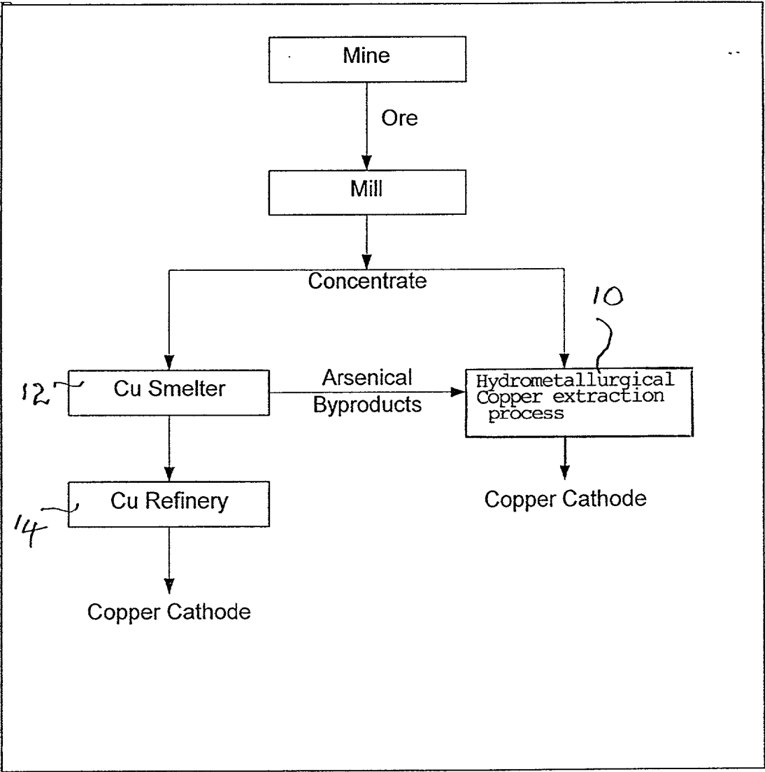
Figure 1 – Overall Process Flowsheet, Copper Ore with Arsenic to Copper Metal
