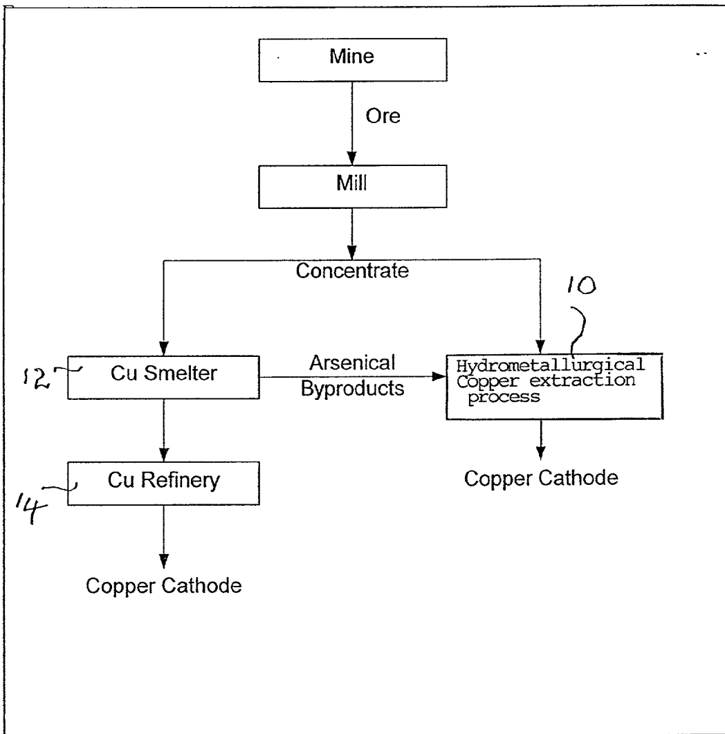
– Overall Process Flowsheet, Copper Ore with Arsenic to Copper Metal
