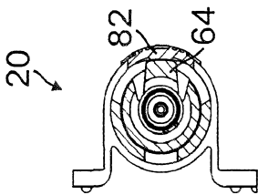
FIG. 2 SECTION C-C
