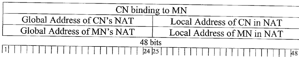
Figure 7 (Prior Art)
